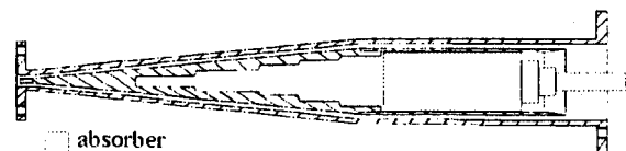
Fig. 4 TM_{0n} waveguide-mode launcher
