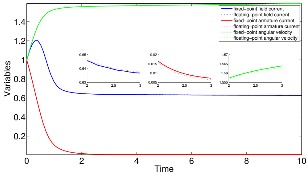
Figure 4.10: DC Motor Using Floating-point and Fixed-point Controller with zoomed-in view for 2 to 3 seconds.
