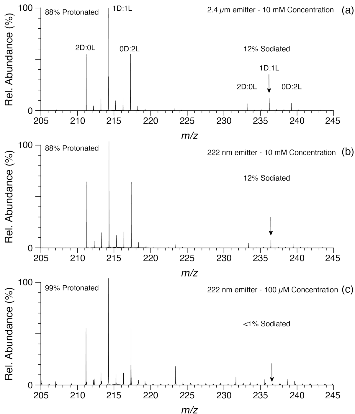
Figure S1. Electrospray ionization mass spectra of an equimolar concentration of D-serine and 2,3,3-d 3 -L-serine at in 49.95:49.95:0.1 water:methanol:acetic acid at 10 mM total concentration with a) a 2.4 \mu\text{m} emitter, b) a 222 nm emitter and c) a 100 \mu\text{M} total concentration with a 222 nm emitter.
