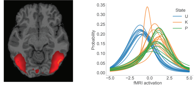
Figure 3: Topography and posterior predictive distributions for MRI emissions from most informative component. Individual traces show the distributions for each fold of the cross validation.
