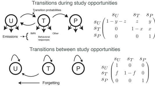
Figure 1: Structure of Atkinson’s (1972) three state Markov model showing latent memory states, the allowable transitions between them during learning and forgetting, and the parameters governing the state transitions.
