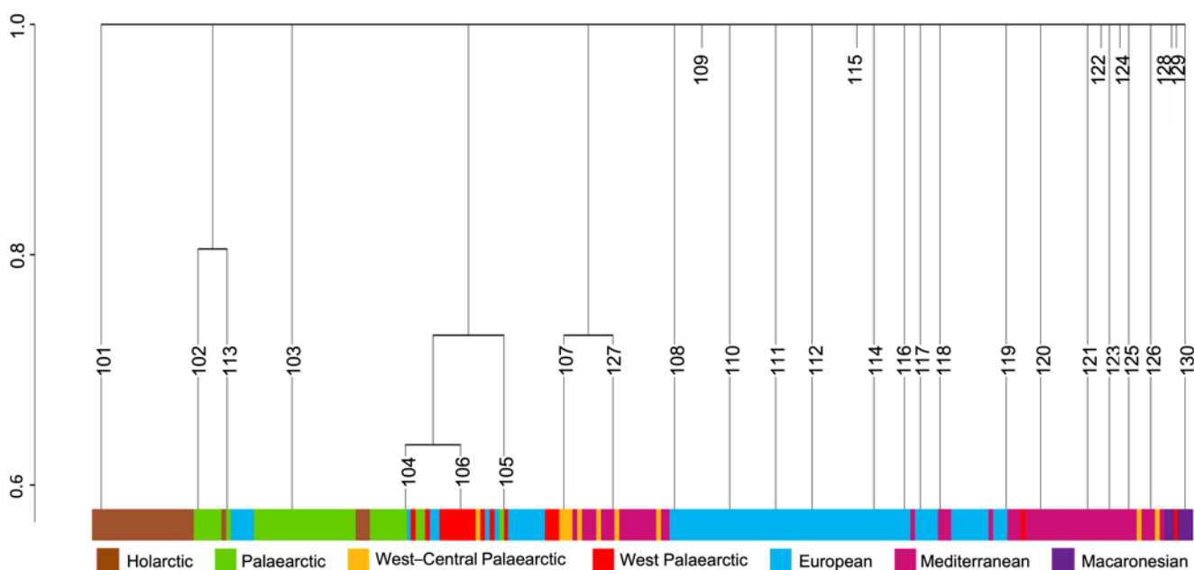
Figure 2. Dendrogram of classification C1 (Baroni-Urbani and Buser index 2, complete linkage clustering). Only branches above the level of significance are displayed (the complete dendrogram including species labels is in the Supplementary Material Fig. S1). The numbers of significant C1 clusters are displayed on the dendrogram branches (corresponding to the text and Supplementary Material Figs S1 and S3). The coloured band beneath the dendrogram consists of bars for each species according to the chorotype group to which the species belongs.
