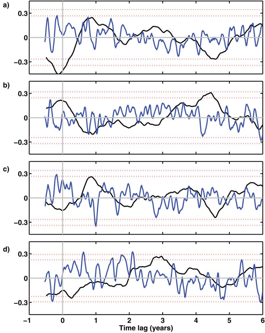
Figure 6. Correlations between the ENSO index (black line) or the SAM index (blue line) and (a) \mathcal{H}_{400} , (b) \phi_{FF} , (c) \mathcal{H}'_S , and (d) \mathcal{H}'_S . Positive time lags indicate that the ENSO or SAM index precedes the XBT transect. Red dotted lines indicate the 0.95 and 0.99 significance levels.
