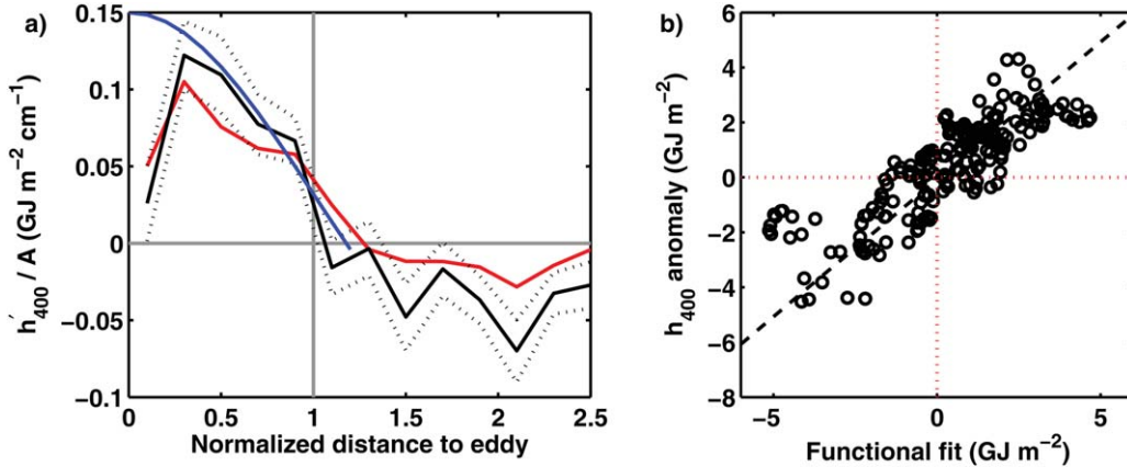
Figure 9. (a) The heat content anomaly ( h'_{400} ) associated with the eddy is a function of distance from the eddy center, d , and the length scale, R , and amplitude, A , of the eddy. For measurements located within an eddy, h'_{400} was normalized by the amplitude of the eddy; binned averages of h'_{400}/A were computed at d/R ranging from 0.1 to 2.5. Mean (black line) \pm 1 standard error (dotted lines) and median (red) h'_{400}/A decrease from maxima near 0.3 R from the eddy center to 0 at 1\text{--}1.3 R from the center. A truncated Gaussian curve (blue line) as in equation (3) approximates f(r,A) . (b) A scatterplot of h'_{400} against the value of f(r,A) at each measurement point (black circles) and the one-to-one line fit (dashed line).
