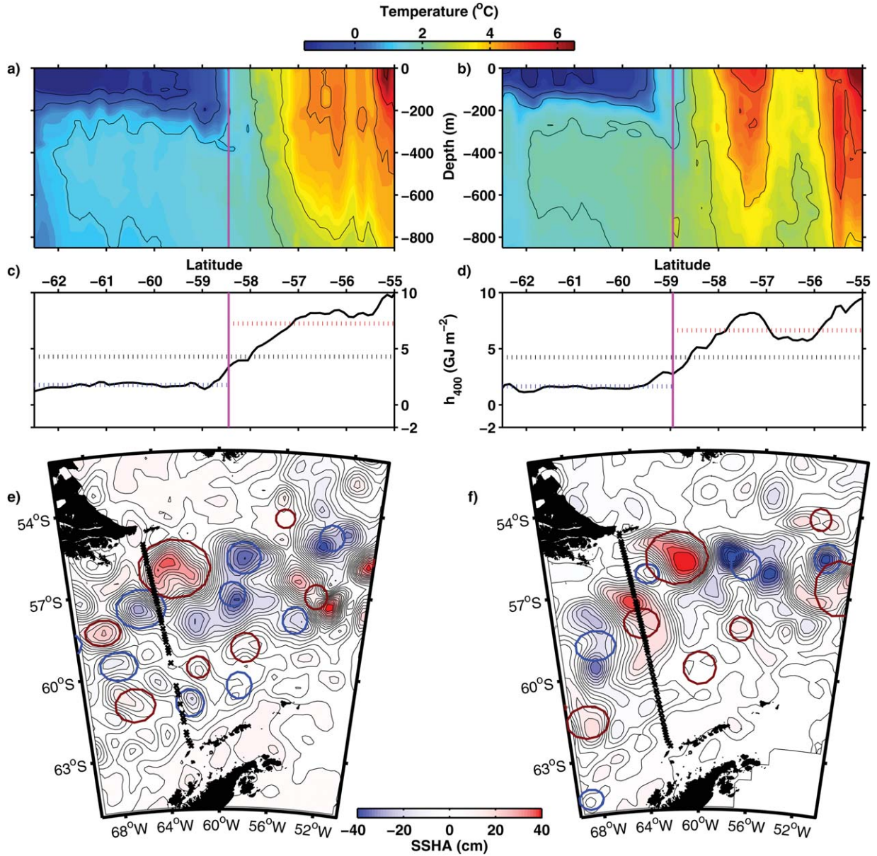
Figure 2. Temperature transects from June cruises in (a) 2006 and (b) 2009. Transects of heat content from 0 to 400 m, h_{400} , across (c) the June 2006 transect and (d) the June 2009 transect with average heat content north of the Polar Front ( \mathcal{H}_N , red dotted line), south of the Polar Front ( \mathcal{H}_S , blue dotted line), and over the entire transect ( \mathcal{H}_{400} , black dotted line). In Figures 2a–2d, the latitude of the Polar Front is indicated by a magenta line. Maps of daily sea surface height anomaly (e) 12 June 2006 and (f) 30 June 2009 and locations of XBT casts (black x). Center location and approximate length scale of cyclonic (blue) and anticyclonic (red) eddies identified in Chelton et al. 's [2011b] database.
