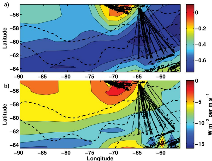
Figure 5. (a) Correlation of NCEP Reanalysis 2 heat flux anomalies ( Q'_{net} ) with meridional wind anomalies. (b) Regression coefficients of Q'_{net} onto meridional wind anomalies. Climatological positions of the ACC fronts (dashed lines) are, from north to south, the Subantarctic Front, Polar Front, and southern ACC Front. Locations of XBT casts (black dots) are indicated.
