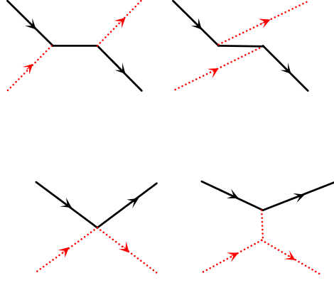
FIG. 1 Lowest order diagrams illustrating the gravitational analog to Compton scattering. Continuous lines indicate a matter particle, short dashed lines a graviton. Consistency of the theory requires that the two bottom diagrams be added to the two on the top.
