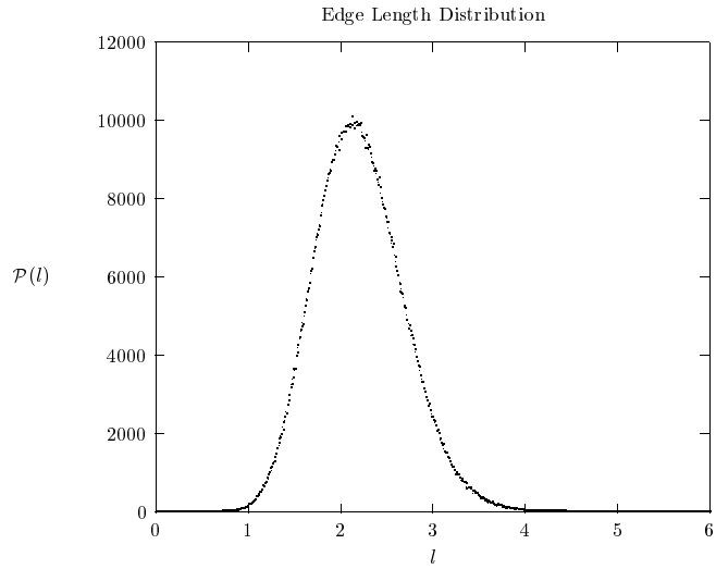
FIG. 33 A typical edge length distribution in the smooth phase for which k < k_c , or G > G_c . Note that the lattice gravitational measure of Eq. (406) cuts off the distribution at small edge lengths, while the cosmological constant term prevents large edge lengths from appearing.
