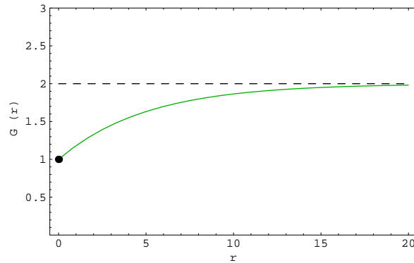
FIG. 42 Schematic scale dependence of the gravitational coupling G(r) , from Eq. (721) valid for \nu = 1/2 . The gravitational coupling rises initially like a power of r , and later approaches the asymptotic value G_\infty = (1 + a_0)G for large r . The behavior for other values of \nu > 1/3 is similar.
