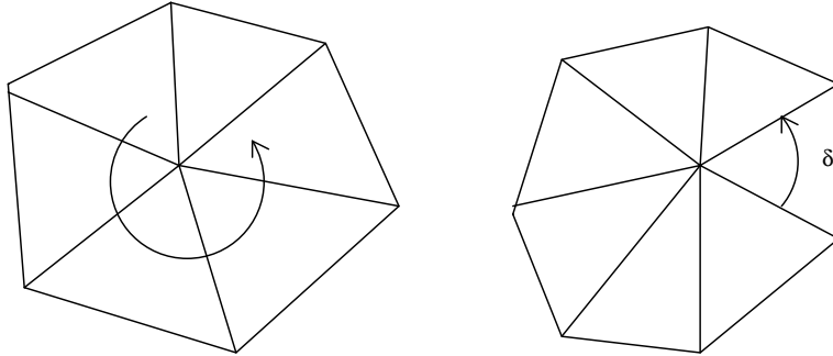
FIG. 12 Illustration of the deficit angle \delta in two dimensions, where several flat triangles meet at a vertex.
