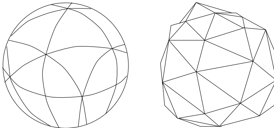
FIG. 9 Polyedral approximation to a sphere.
