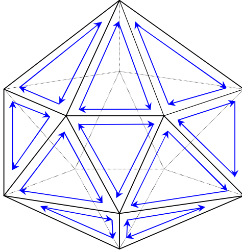
FIG. 29 Elementary closed surface tiled with parallel transport polygons, here chosen to be triangles for illustrative purposes. For each link of the dual lattice, the elementary parallel transport matrices \mathbf{R}(s, s') are represented by an arrow. In spite of the fact that the (Lorentz) matrices \mathbf{R} fluctuate with the local geometry, two contiguous, oppositely oriented arrows always give \mathbf{R}\mathbf{R}^{-1} = 1 .
