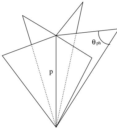
FIG. 15 Angles appearing in the Regge equations.
