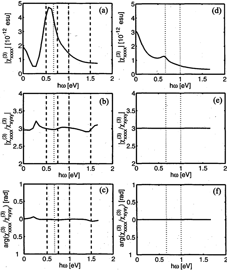
Figure V.15: Models for the nonlinear response of \text{Sr}_2\text{CuO}_2\text{Cl}_2 . (a)–(c) and (d)–(f) show |\chi_{xxxx}^{(3)}| , \kappa_{xx}/\kappa_{xy} and phase difference \delta for two different models, respectively. For (a)–(c) the model incorporates the charge transfer p_{x,y} states at 2 eV, a 3d_{xy} state at 1.35 eV, a 3d_{3z^2-r^2} state at 1.5 eV and finally an s state at 3 eV. Each level has a particular broadening, and the ground state is of 3d_{x^2-y^2} character. (d)–(f) are calculated using only the charge transfer state as an excited state. The apparent resonance at \hbar\omega=0 eV in (d) is an artifact.
