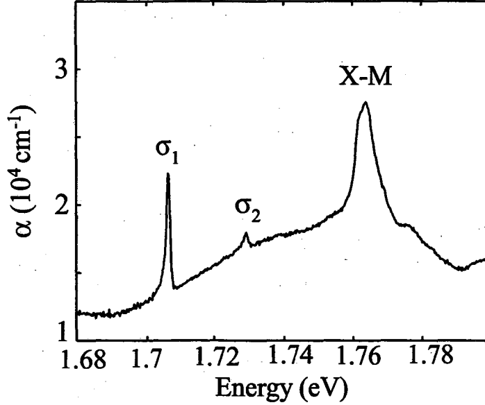
Figure IV.1: Linear absorption spectrum of \text{Cr}_2\text{O}_3 in the vicinity of the exciton magnon band. The two sharp features \sigma_1, \sigma_2 to the left are the optically weakly allowed {}^4A_2 \rightarrow {}^2E excitons. The stronger absorption feature X-M to the right is the magnetic side band, or exciton-magnon compound object.
