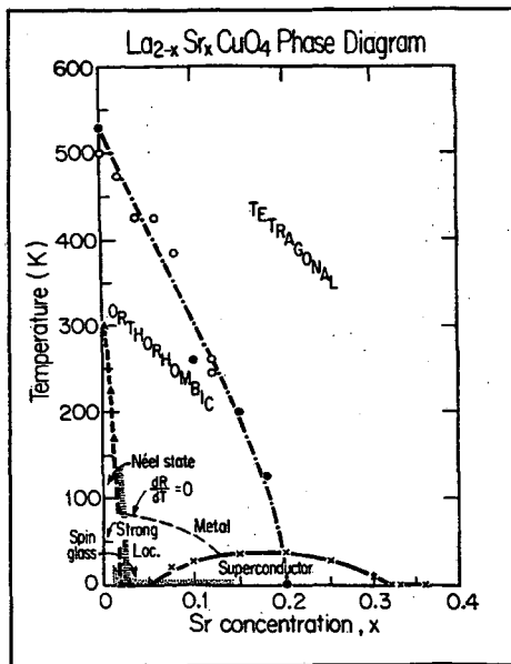
Figure II.4: Phase diagram of cuprate \text{La}_{2-x}\text{Sr}_x\text{CuO}_4 . From Ref. [46].
