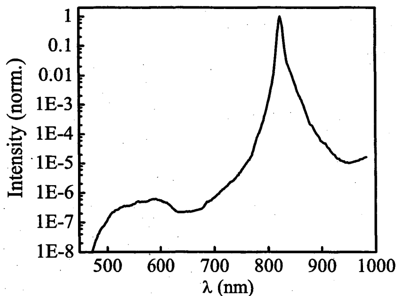
Figure III.6: Spectrum of the white light continuum. The resolution at the long-wavelength side is limited by the spectrometer. The spectrum shows the typical plateau on the high-energy side [10].
