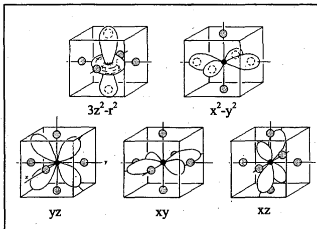
Figure II.1: 3d orbitals. The five-fold degeneracy is partially lifted in a cubic environment. A tetragonal distortion (not shown here) would further reduce the degeneracy and cause a splitting into (xz,yz) , xy , 3z^2-r^2 and x^2-y^2 states (listed by increasing electron energy ).
