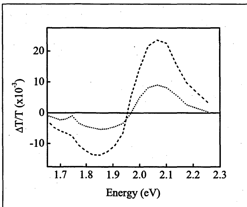
Figure V.18: Comparison between photoinduced response at 2.1 eV (dotted line) and 3.1 eV (dashed line) pump energy. In both cases the excitation density is again 7 \times 10^{18} \text{ cm}^{-3} , or 8 \times 10^{-4} \text{ Cu}^{-1} . T=15 K
