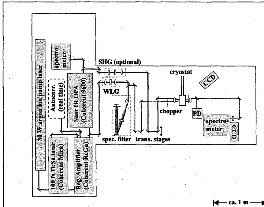
Figure III.3: Layout of the optical table. Autocorr.: real time and stepper motor autocorrelator, non-collinear geometry. SHG: 1 mm BBO crystal for frequency doubling of the near-IR OPA (optional). WLG: Supercontinuum generation in a 3 mm sapphire crystal. PD: UV enhanced Si large area photo diode for time-resolved measurements. A CCD camera is used to monitor the beam positions on the sample. Not shown are various filters and polarization optics used in different experiments.
