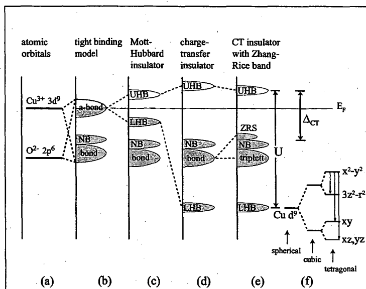
Figure II.3: Schematic density of states for a transition metal oxide. (a) atomic orbitals. (b) in a single-electron tight binding picture the oxygen-like bonding bands (bond) and non-bonding band (NB) lie below E_F , whereas the antibonding (a-bond) bands are close to E_F . (c) on-site Coulomb interaction splits the conduction band into lower (LHB) and upper (UHB) Hubbard bands. (d) for \Delta_{CT} < U , the material is a charge transfer insulator. \Delta_{CT} is the gap between the highest oxygen-like state and the UHB. (e) Cu 3d-O 2p hybridization creates Zhang-Rice singlets (ZRS, see chapter V) just below the UHB. (f) charge-neutral on-site excitations can occur within the LHB, and are influenced by the crystal symmetry
