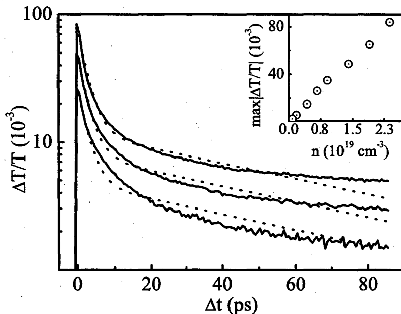
Figure V.19: Time-resolved spectroscopy at 3.1 eV pump and 2.1 eV probe energy for three different excitation densities ( 0.3, 1.5, 2.3 \times 10^{19} \text{ cm}^{-3} from bottom to top). The dashed lines represent global best fits to a double exponential decay with \tau_1 = 2.6 ps and \tau_2 = 70 ps. The inset shows the linear power dependence of the instantaneous signal as a function of the carrier density n . Sample temperature 15 K
