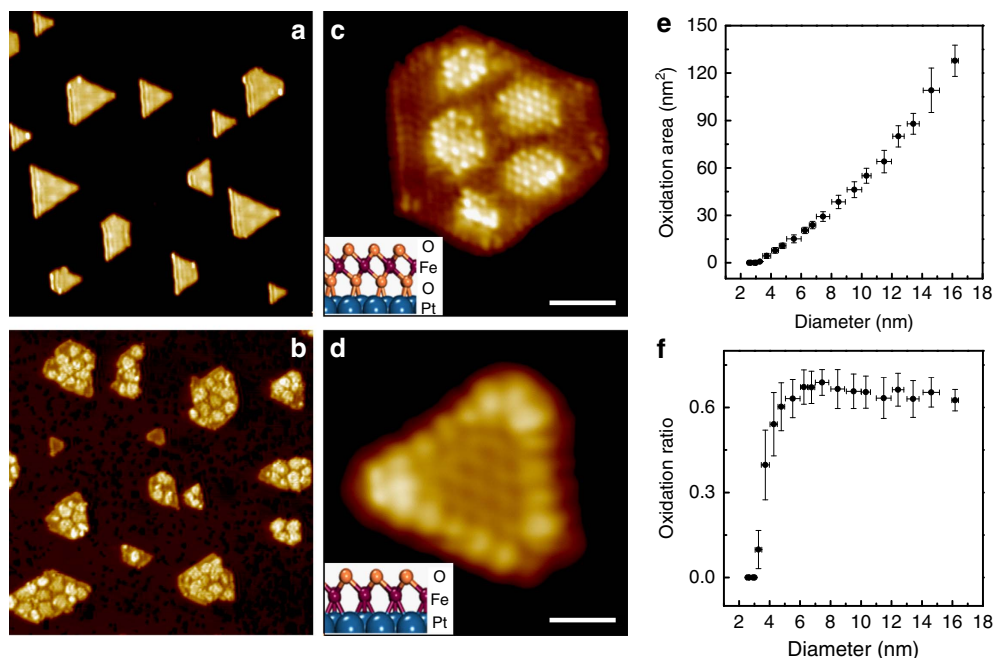
Figure 1 | The size-dependent oxidation kinetics of FeO nanostructures(NSs) on Pt(111). (a,b) STM images (50 nm × 50 nm) of the typical surface of as-prepared FeO NSs on Pt(111) (a) and the FeO/Pt(111) surface after the annealing in 1 \times 10^{-5} mbar O_2 at 500 K for 10 min (b). Most FeO NSs were oxidized to form FeO_2 domains, except for FeO NSs with an equivalent diameter d < 3.2 nm. Here, the FeO NS is treated as a circle and the equivalent diameter is defined as d = 2 \times \sqrt{S/\pi} , where S is the NS surface area. (c,d) Atomic STM images of an oxidized FeO NS ( d = 6.2 nm) with the formation of FeO_2 domains and an FeO NS ( d = 2.1 nm) remaining the FeO phase, respectively. The structural models (side view) of FeO_2 and FeO on Pt(111) are shown in the insets. STM images were taken at 230 K and scanning parameters (sample bias: V_s ; tunneling current: I_t ) are (c) V_s = +104 mV, I_t = 3.5 nA; (d) V_s = +53 mV, I_t = 2.1 nA. Scale bars are 2 nm in c and 1 nm in d. The area of FeO_2 domains ( S_{FeO_2} ) on each NS, as well as the NS surface area ( S ), are measured over 247 FeO islands on the same surface. (e,f) plot the oxidation area ( S_{FeO_2} ) and the oxidation ratio ( S_{FeO_2}/S ) of individual FeO NSs as a function of d , where the size range of FeO NSs and the s.d. of S_{FeO_2} and S_{FeO_2}/S are represented by error bars.
