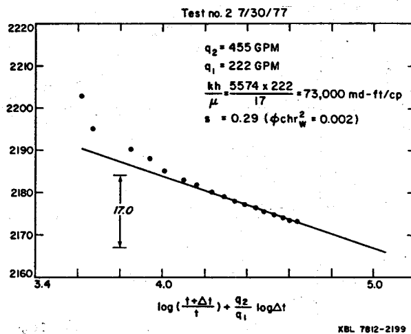
Fig. 8. Test segment no. 2, 18-28 production test.
