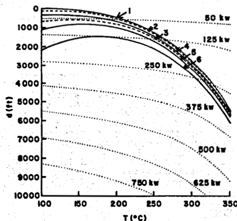
FIGURE 3. MINIMUM DEPTH REQUIRED TO PREVENT STEAM FORMATION IN A PUMPED AQUIFER HOT WATER STORAGE WELL AT VARIOUS STORAGE TEMPERATURES AND A FLOW RATE OF 500 GAL/MIN. ALSO SHOWN (DOTTED CURVES) IS MAXIMUM DEPTH, AS A FUNCTION OF TEMPERATURE, FROM WHICH A PUMP OF THE INDICATED POWER, CAN LIFT THE WATER.
