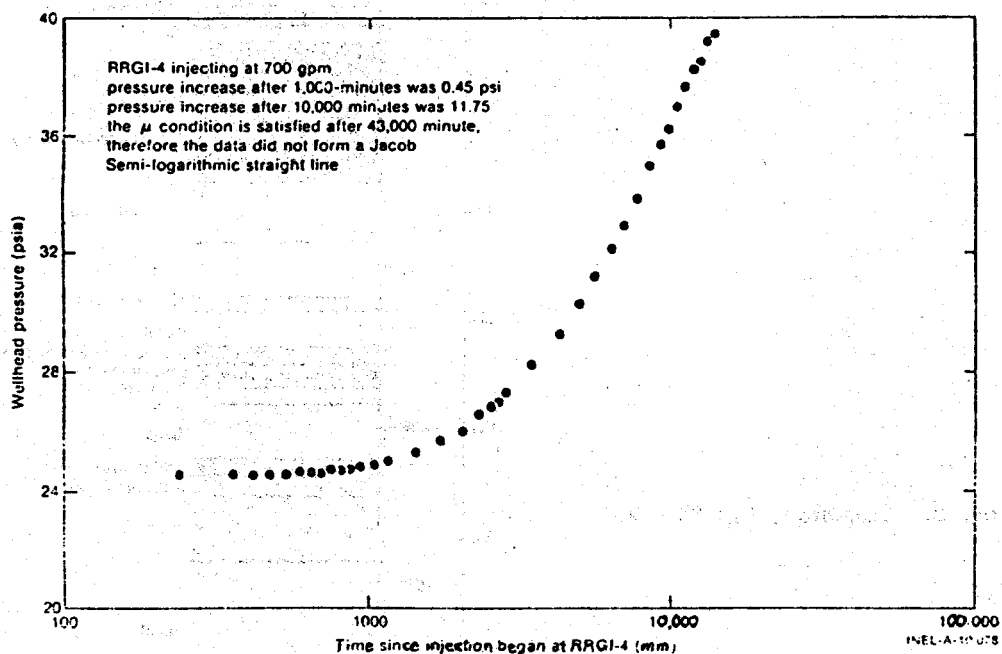
Fig. 5. Pressure buildup at USGS-3 during May 30, 1978, injection test at RRG-4.
