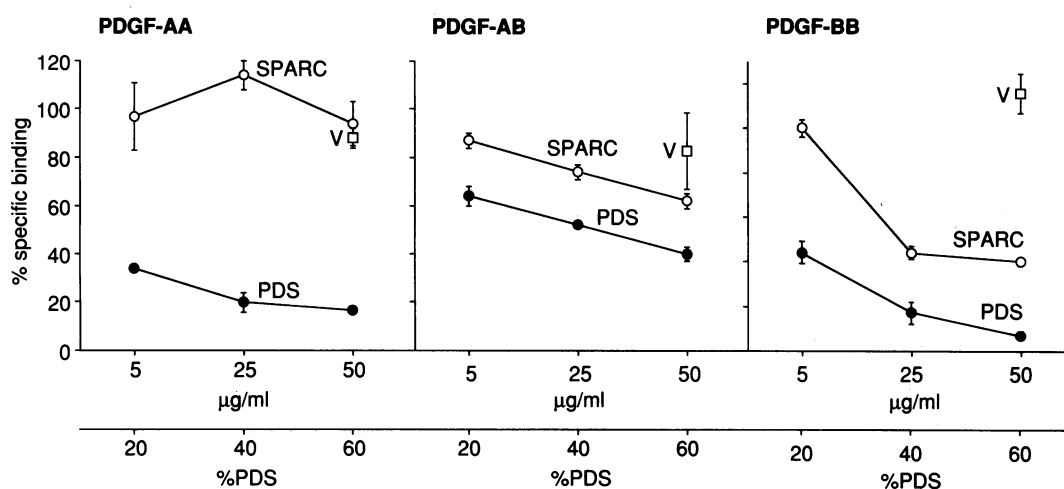
FIG. 4. SPARC inhibits the binding of PDGF-BB and PDGF-AB, but not PDGF-AA, to human dermal fibroblasts. ^{125}\text{I} -PDGF dimeric forms were preincubated with SPARC, human plasma-derived serum (PDS), or type V collagen (V), and specific binding to human skin fibroblasts was subsequently measured. Addition of SPARC had no effect on the binding of PDGF-AA to cells ( Left ). However, SPARC inhibited the binding of PDGF-AB ( Center ) and PDGF-BB ( Right ) in a dose-dependent fashion. Type V collagen had no effect on the binding of any dimeric form of PDGF, and plasma-derived serum inhibited the binding of all three dimeric forms. Data represent the mean \pm SEM of triplicate determinations, and the experiment shown is representative of three separate experiments. Samples were checked in a sequential radioreceptor assay and shown to be free of endogenous PDGF (data not shown).
