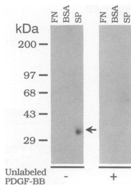
FIG. 2. ^{125}\text{I} -PDGF-BB binds to SPARC immobilized on nitrocellulose but not to fibronectin or BSA. SPARC (SP, 500 ng), BSA (2 \mu\text{g} ), fibronectin (FN, 2 \mu\text{g} ), and molecular size standards were resolved by SDS/PAGE, transferred to nitrocellulose, and incubated with ^{125}\text{I} -PDGF-BB (10 ng/ml). PDGF-BB bound only to SPARC (arrow). The binding of iodinated PDGF-BB was eliminated when 100-fold excess unlabeled PDGF was preincubated with the blot prior to the addition of ^{125}\text{I} -PDGF-BB.
