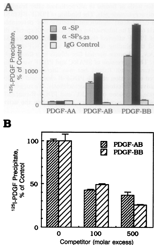
FIG. 1. Anti-SPARC antibodies specifically immunoprecipitate PDGF-BB and PDGF-AB but not PDGF-AA. (A) 125 I-PDGF-SPARC complexes were precipitated by two independently derived anti-SPARC antibodies ( \alpha SP; \alpha SP 5-23 ) but not by a preparation of normal rabbit IgG (IgG control). Control binding of 125 I-PDGF in the absence of SPARC was defined as 100% and was equivalent to 2.06 fmol of PDGF-AA, 0.07 fmol of PDGF-AB, and 0.36 fmol of PDGF-BB. All assays were performed in triplicate, and data were plotted as percentage of control ( \pm SEM). (B) Unlabeled PDGF-AB and PDGF-BB inhibit immunoprecipitation of 125 I-PDGF-SPARC complexes. SPARC was preincubated with 100-fold (300 ng) or 500-fold (1.5 \mu g) excess unlabeled PDGF for 4 hr before incubation with labeled PDGF. Binding to SPARC in the absence of nonradiolabeled competitor was defined as 100%.
