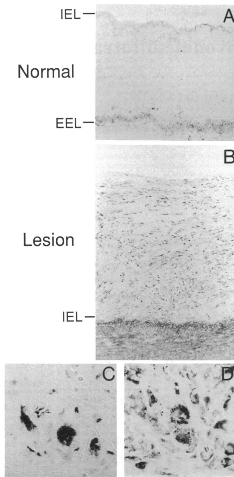
FIG. 6. Expression of PDGF-B chain and SPARC is induced in lesions of atherosclerosis. Sections of vessels from normal (A) or hypercholesterolemic (B–D) monkeys were incubated with antibodies to PDGF-B chain (C) or to SPARC (A, B, and D). Reaction product (dark stain) was visualized by an avidin–biotin–peroxidase technique. Normal vessels contained no PDGF-positive cells (data not shown), and immunoreactivity for SPARC was limited and confined to areas adjacent to the internal (IEL) and external (EEL) elastic laminae. Expression of SPARC was increased in advanced atherosclerotic lesions and was observed in most medial smooth muscle cells and in scattered cells of the neointima (B). Examination of adjacent sections of the advanced lesion at higher power demonstrated localized expression of PDGF-B chain in intimal cells (C), previously identified as macrophages, and expression of SPARC by apparently the same cells and in additional neointimal cells (D), identified in adjacent sections as smooth muscle cells (data not shown). ( \times 36 in A and B; \times 225 in C and D.)
