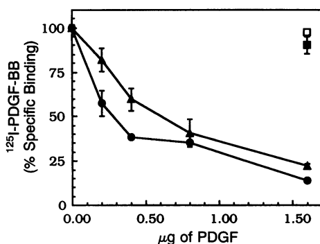
FIG. 5. Competitive inhibition of the binding of ^{125}\text{I} -PDGF-AB and -BB to SPARC. SPARC (500 ng) was incubated 4 hr with the indicated amounts of PDGF and then with 15 ng of ^{125}\text{I} -PDGF-BB. ^{125}\text{I} -PDGF–SPARC complexes were precipitated with antibody to SPARC-(5–23) peptide. Control binding of ^{125}\text{I} -PDGF-BB to normal rabbit IgG (<12% of PDGF–SPARC binding) was used to evaluate nonspecific binding. All points were determined in triplicate and plotted as percent specific binding ( \pm SEM). In this experiment, 3 ng of ^{125}\text{I} -PDGF-BB was bound to SPARC in the absence of competitive inhibitor. \blacktriangle , PDGF-AB; \bullet , PDGF-BB; \square , PDGF-AA short ; \blacksquare , PDGF-AA long .
