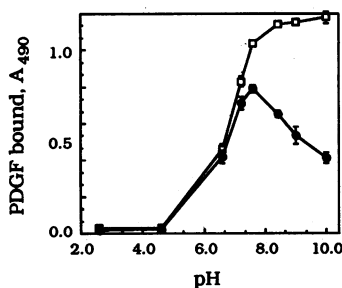
FIG. 3. Binding of PDGF-BB to immobilized SPARC is pH-dependent. Microtiter wells coated with SPARC were blocked and pre-equilibrated for 1 hr in universal buffers of a constant ionic strength (conductance, 15 mS) that were adjusted to pH values between 2.6 and 10.0. PDGF-BB diluted to a final concentration of 50 ng/ml was incubated with SPARC for 2 hr in the same buffers. All wells were re-equilibrated to pH 7.7 and total binding ( \square ) was determined in triplicate ( \pm SEM) at each pH for wells containing SPARC and for control wells containing blocking agent alone with anti-PDGF antibodies. Specific binding ( \bullet ) represents the total protein bound minus the nonspecific protein bound to control wells. Separate determinations were performed to verify that a constant amount of SPARC remained immobilized at all pH values and that recognition of PDGF by anti-PDGF did not change with treatment (data not shown).
