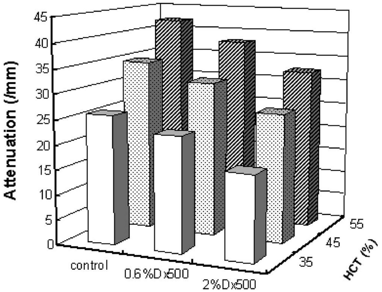
Fig. 2. Summary of attenuation in the blood at HCT=35%, 45%, and 55% without and with Dx500 at a flow rate of 5 mm/sec ( n=3 ).
