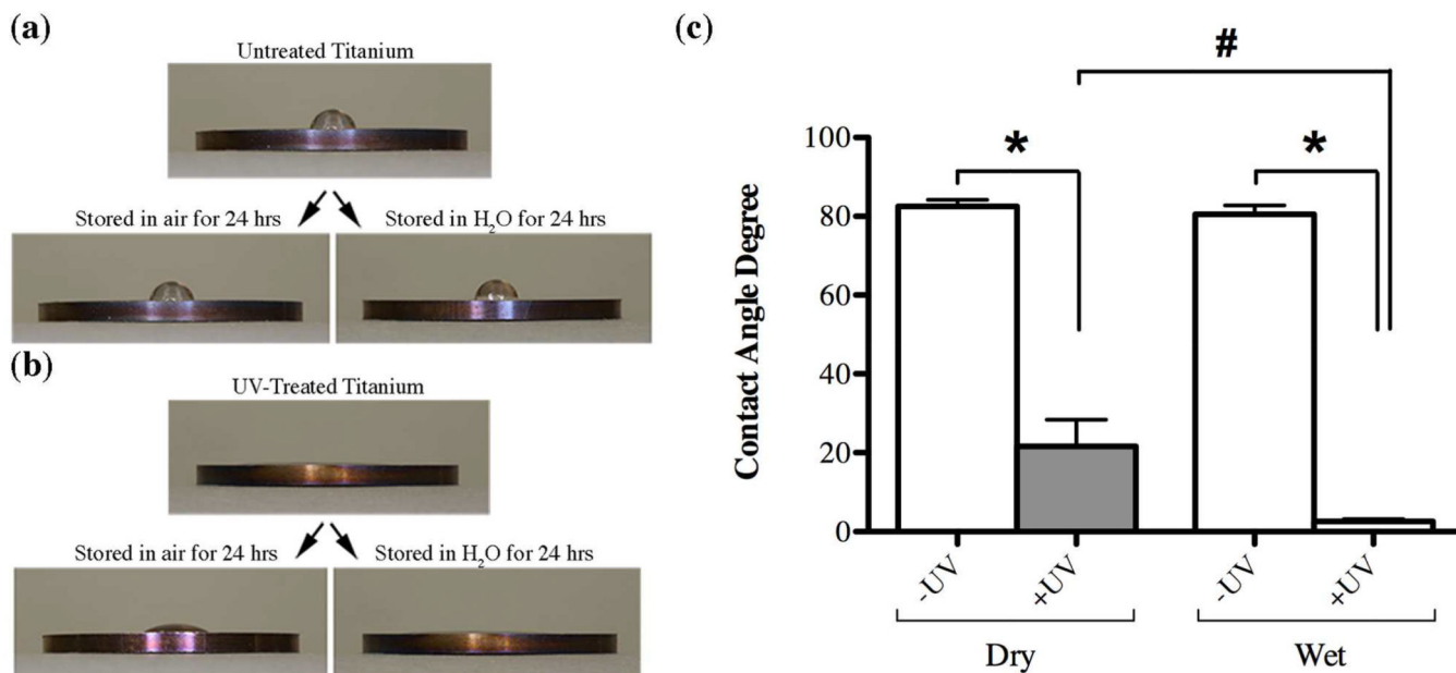
Fig. 2. Measurement of the contact angle of 10µl ddH 2 O to evaluate changes in hydrophilicity of titanium discs surfaces (a) without and (b) after UV-photofunctionalization treatment as well as after subsequent storage in air or a liquid environment for 24 hours. Comparison of contact angles values (c) between untreated (white bars, - UV) and UV-treated (gray bars, +UV) after storage in air (Dry) or a liquid environment (Wet). Statistically significant differences are indicated as: * p < 0.0001 , # p = 0.0042 . Data represent the mean \pm SD of triplicate data from one independent experiment.
