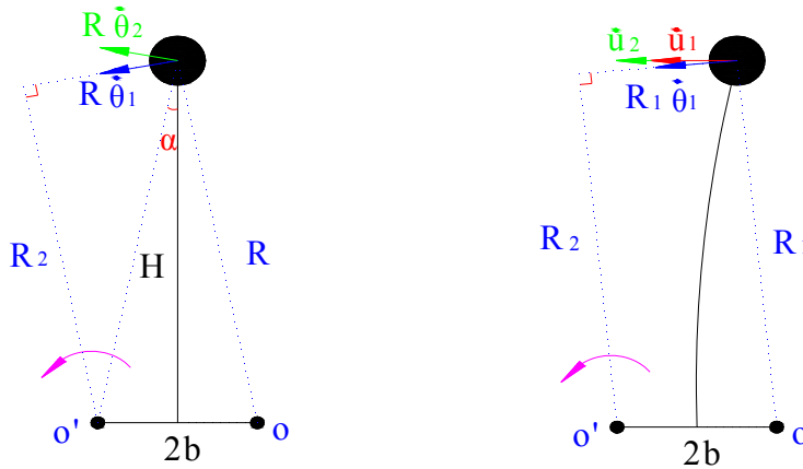
(a) Rigid column case (b) Deformable column case
