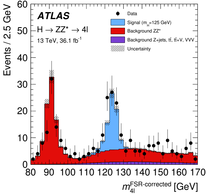
Figure 1: Four-lepton invariant mass distribution of the selected events before the m_{4l} requirement, corrected for final-state radiation (FSR). The error bars on the data points indicate the statistical uncertainty. The SM Higgs boson signal prediction is obtained from the samples discussed in Section 3. The backgrounds are determined following the description in Section 6. The uncertainty in the prediction is shown by the hatched band, calculated as described in Section 9.
