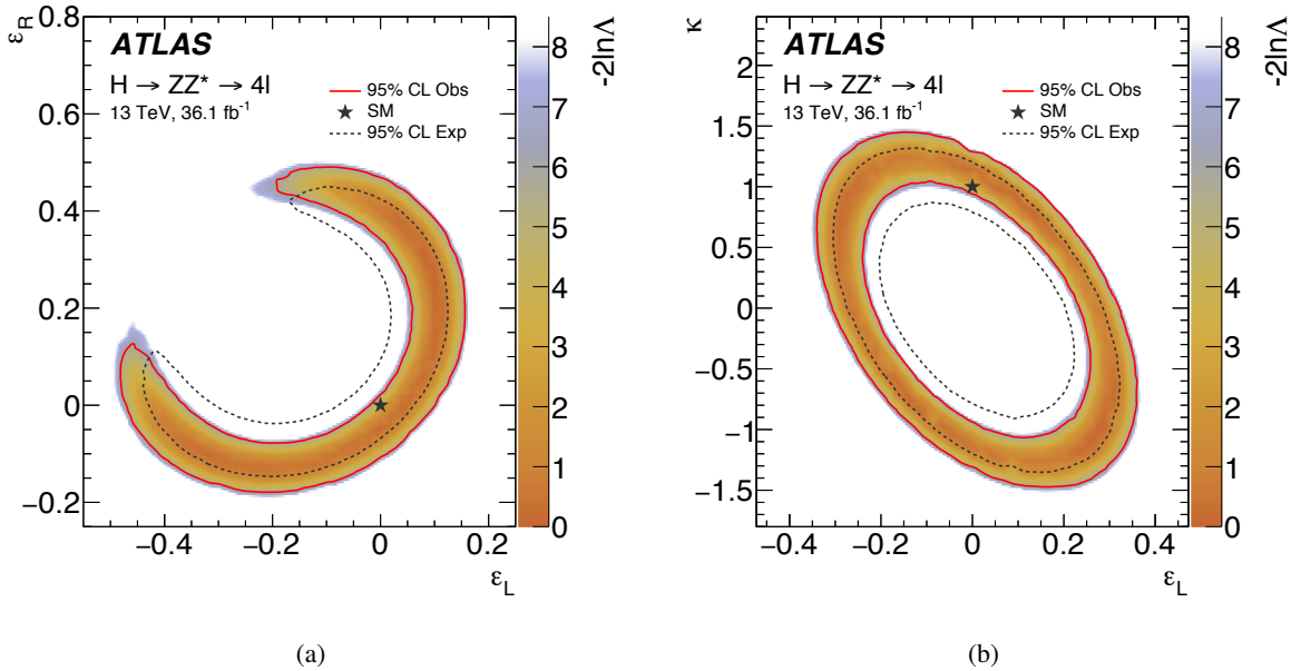
Figure 11: Limits on modified Higgs boson decays within the framework of pseudo-observables [15, 79]. In (a), the limits are extracted in the plane of \varepsilon_{\text{L}} and \varepsilon_{\text{R}} , which modify the contact terms between the Higgs boson and left- and right-handed leptons, assuming lepton-flavour universality. In (b), the tested parameters are \varepsilon_{\text{L}} and \kappa . The latter modifies the coupling of the Higgs boson to Z bosons. The allowed observed area at the 95% CL is surrounded by the red solid line. This can be compared to the SM prediction, which is indicated by the black star and the black dotted line. The coloured scale indicates the values of -2 \ln \Lambda .
