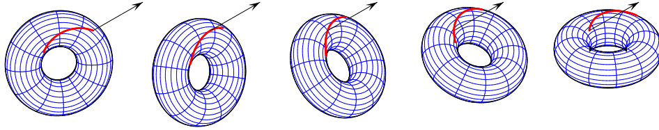
Figure 6: The toolpath (30) for \xi \in [\frac{1}{2}, \frac{3}{2}] on the torus (29) for the case of an orientable-table machine in Example 2. The position and orientation of the torus vary continuously, such that the surface normal (shown as an arrow) at the tool contact point is a fixed vector in the machine coordinate system.
