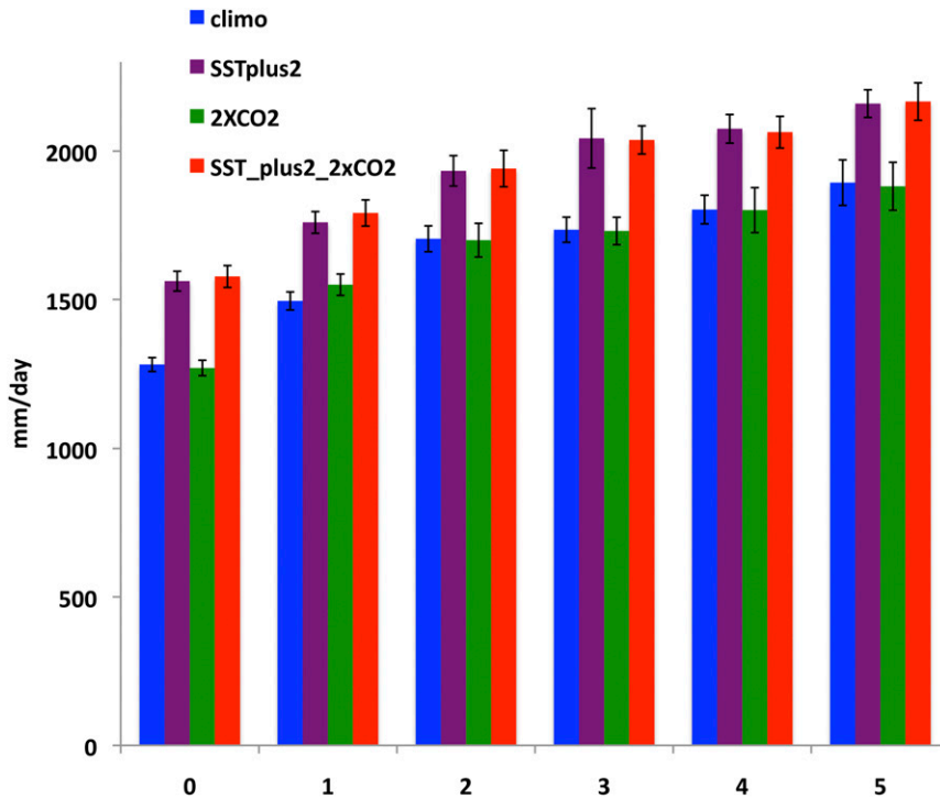
FIG. 7. Global average maximum instantaneous tropical storm precipitation as a function of intensity on the Saffir-Simpson scale simulated by the 0.23^\circ \times 0.31^\circ version of CAM5.1 in the U.S. CLIVAR HWG configurations. Error bars show the 5%–95% confidence interval. Units: \text{mm day}^{-1} .
