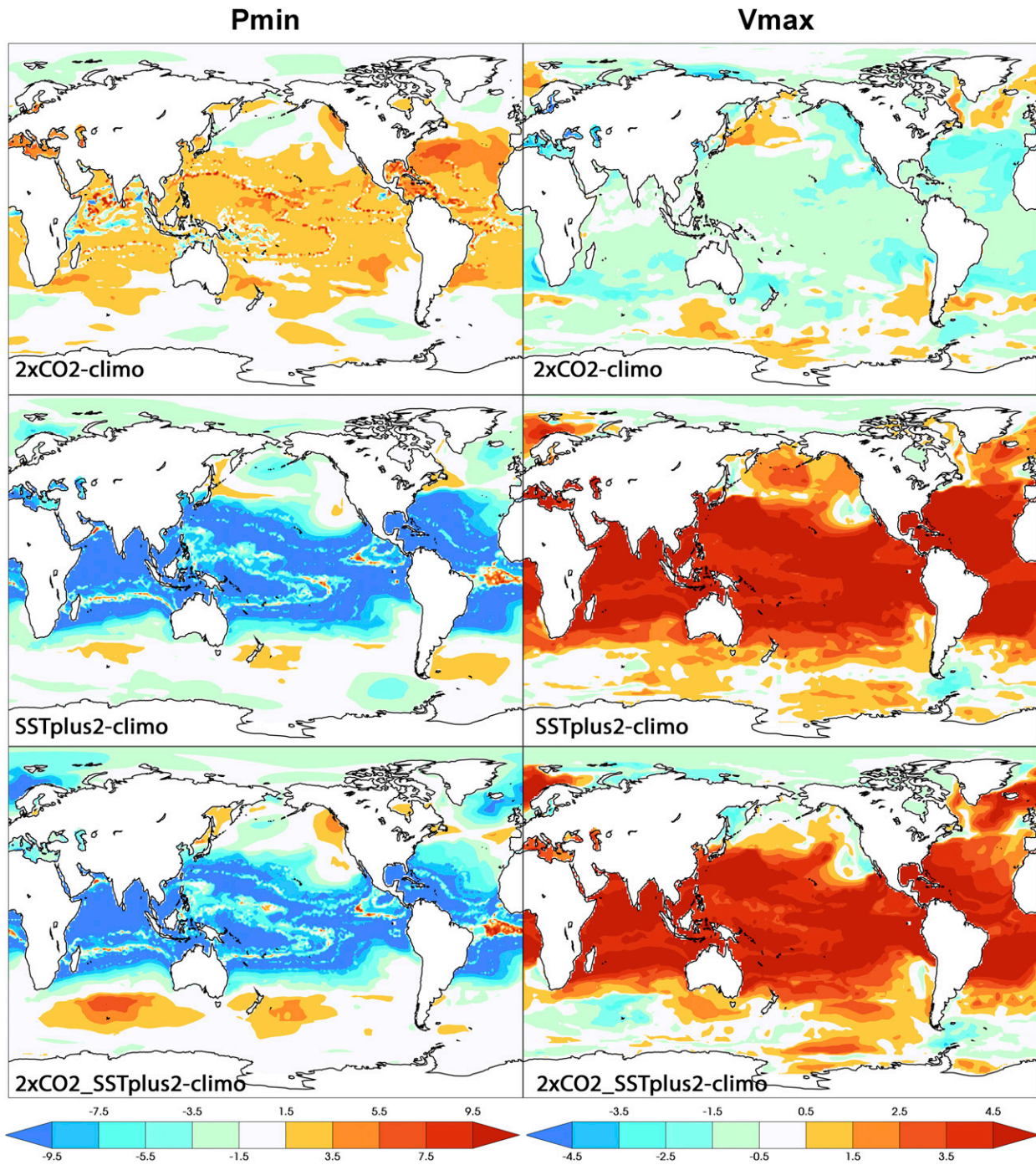
FIG. A2. Difference in annualized maximum potential intensity metrics of the perturbed U.S. CLIVAR HWG experiments from the CLIMO experiment produced by the 0.9^\circ \times 1.3^\circ CAM5.1 configuration: (left) minimum central pressure (hPa) and (right) maximum wind speed ( \text{m s}^{-1} ), for (top) 2xCO2 minus CLIMO, (middle) SSTplus2 minus CLIMO, and (bottom) SSTplus2_2xCO2 minus CLIMO.
