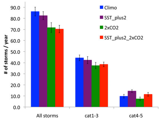
FIG. 4. Global average number of tropical storms, tropical cyclones and intense tropical cyclones per year simulated by the 0.23^\circ \times 0.31^\circ version of CAM5.1 for the four U.S. CLIVAR HWG idealized AGCM configurations. Error bars represent 5%–95% confidence intervals based on interannual variability.
