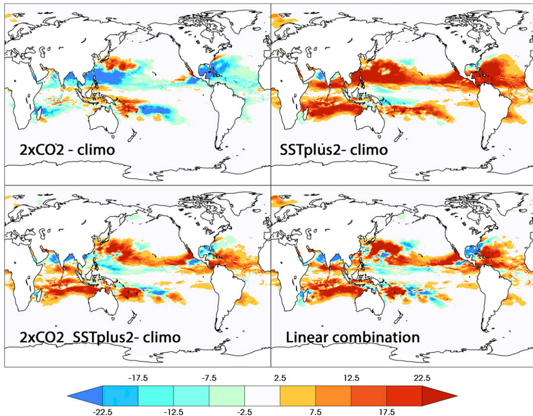
FIG. 10. Difference in annualized genesis potential index of the perturbed U.S. CLIVAR HWG experiments from the CLIMO experiment produced by the 0.23^{\circ} \times 0.31^{\circ} CAM5.1 configuration: (top left) 2xCO_2 minus CLIMO, (top right) SSTplus2 minus CLIMO, (bottom left) SSTplus2_2xCO2 minus CLIMO, and (bottom right) the sum of the two upper panels.
