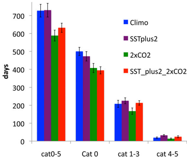
FIG. 6. Annual global average number of storm days simulated by the 0.23^\circ \times 0.31^\circ version of CAM5.1, showing all storm days (categories 0–5), tropical storm days (category 0), tropical cyclone days (categories 1 through 3), and intense tropical cyclone days (categories 4 through 5). Error bars show the 5%–95% confidence interval based on the interannual variability. Units: days.
