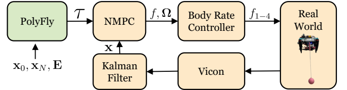
Fig. 8: System architecture for real-world deployment.
