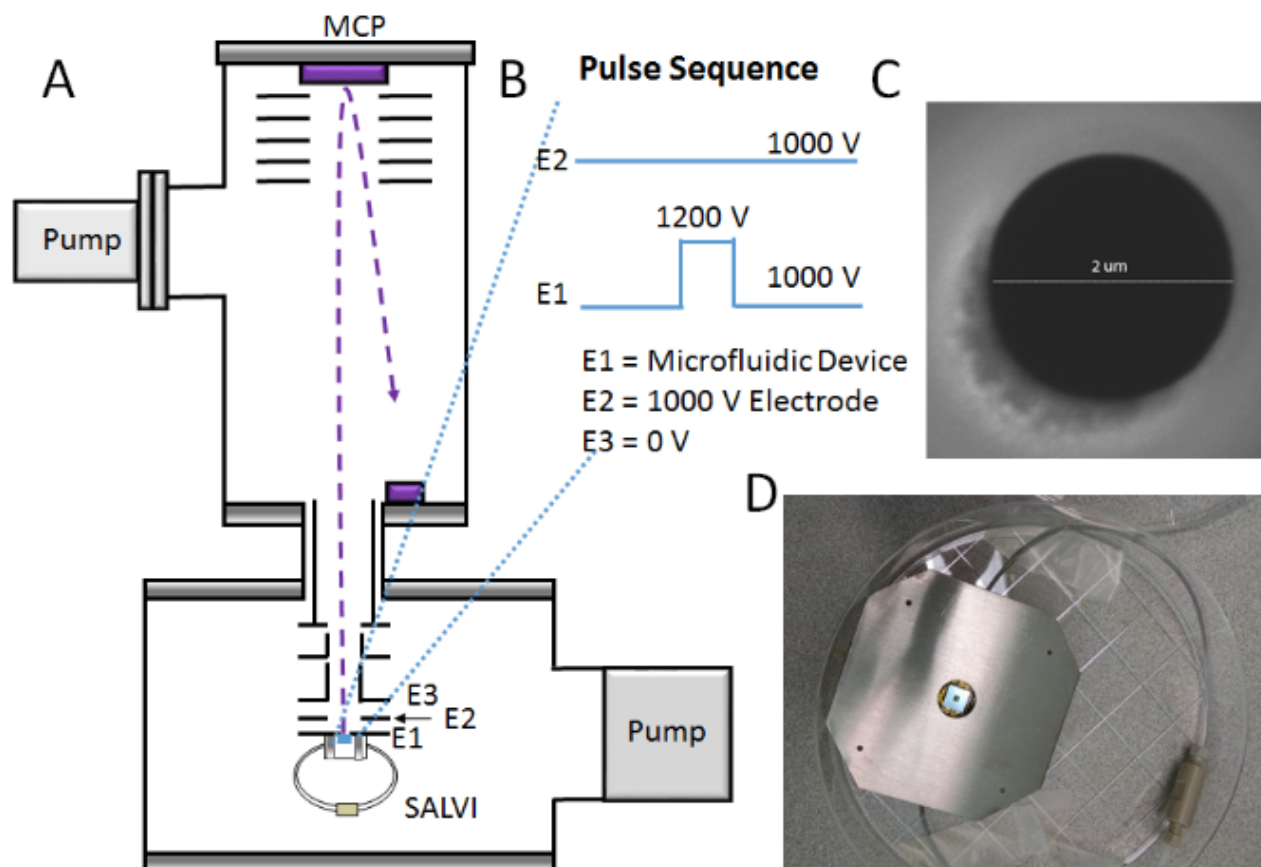
FIG. 1. A schematic showing the SALVI integration to the VUV SPI-MS. Insert A) gives the electrode scheme in the ion optics of ReToF MS with the attached SALVI device, B) provides voltages and the pulse sequence of ReToF MS ion optics, C) a secondary electron image showing the 2 \mu\text{m} diameter hole on the SiN membrane, and D) a photo showing SALVI adapted to the ion optics plate. The SALVI device is attached to the bottom electrode in A. The schematic diagram in A was adapted from Kaiser R.I. et al. 2010 and Góbi, S. et al. 2018. 3,6
