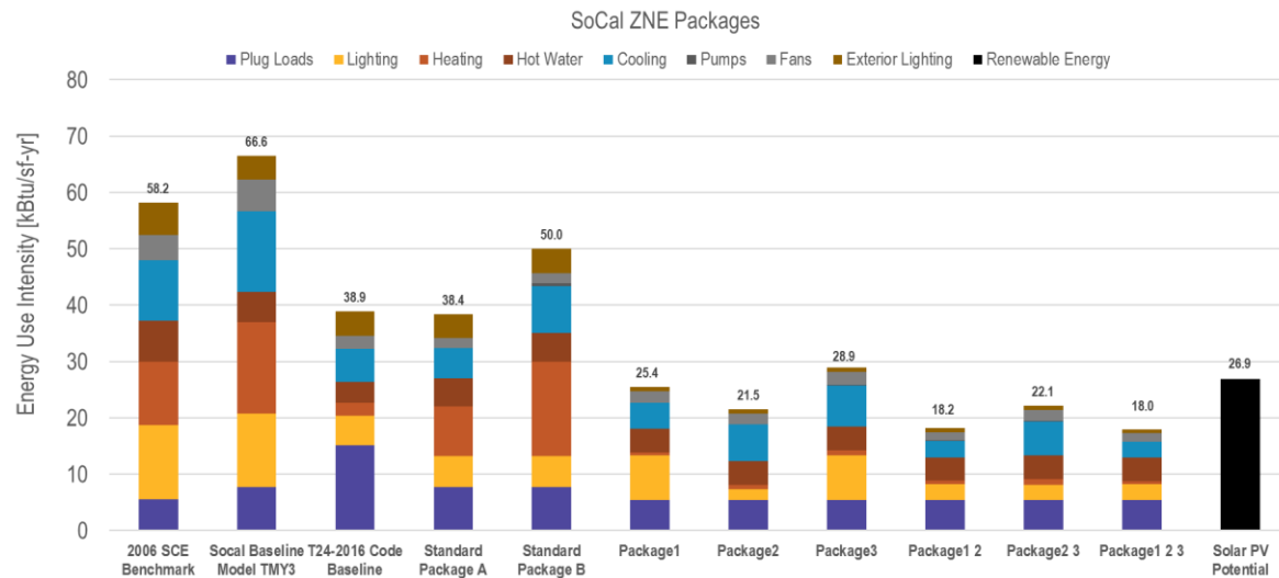
Figure 1b. Southern California ZNE Package Annual Energy Intensity Compared to Onsite PV Production, Existing Building Baselines and Title 24-2016 Minimum Energy Code Compliance
