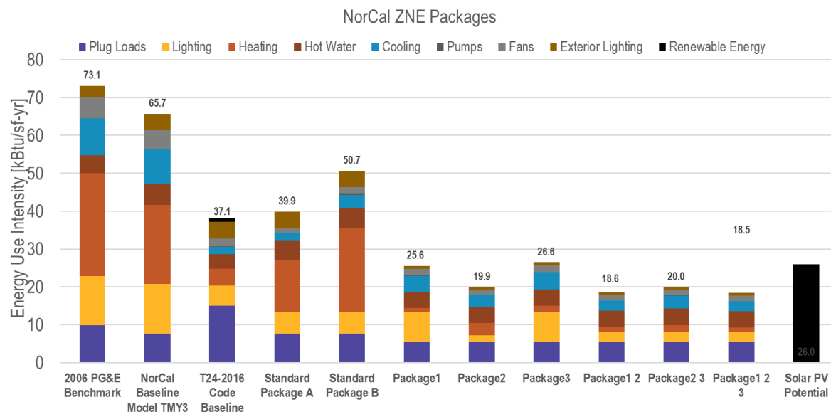
Figure 1a. Northern California ZNE Package Annual Energy Intensity Compared to Onsite PV Production, Existing Building Baselines and Title 24-2016 Minimum Energy Code Compliance
