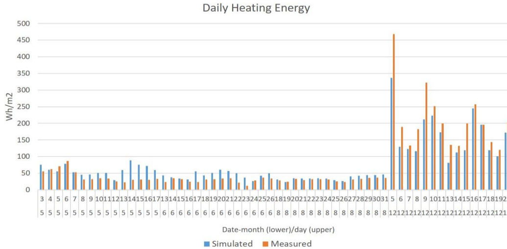
Figure 13. Daily heating energy comparison between simulation and measurement.
