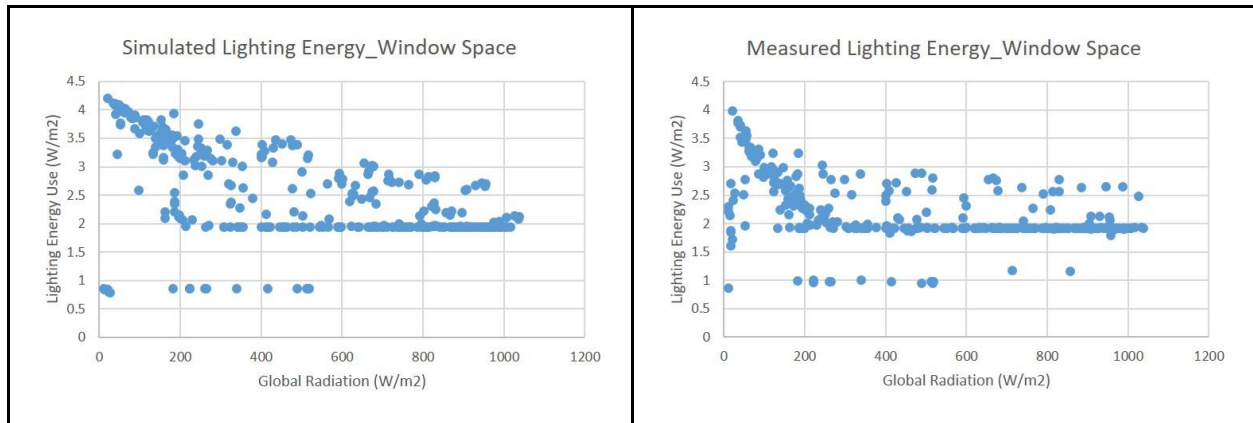
Figure 9. Variation of the window space lighting energy use with global radiation - simulated vs. measured.
