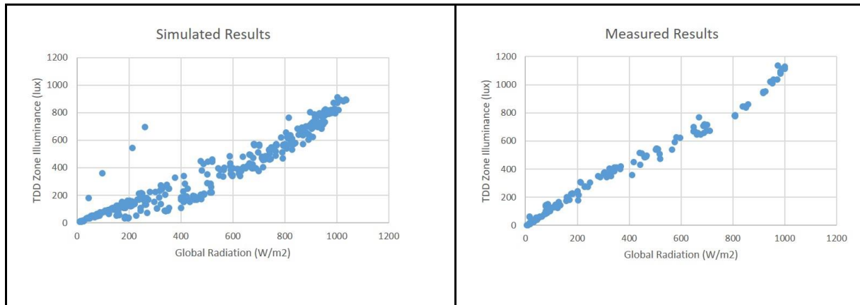
Figure 7. Variation of the TDD space illuminance with global radiation - simulated vs measured.
