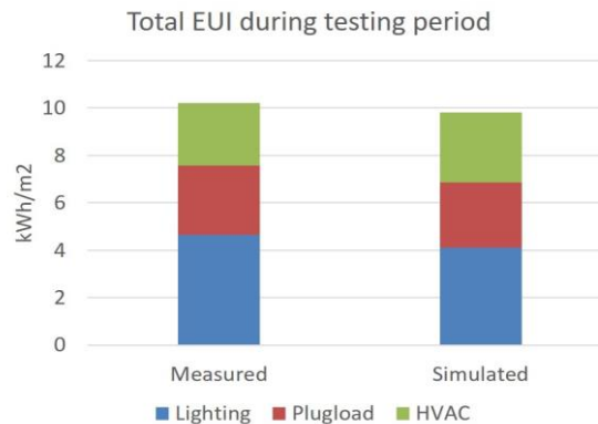
Figure 14. Comparison of total EUI during testing period - simulation and measurement.
