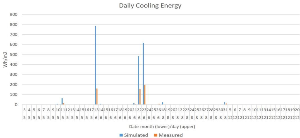
Figure 12. Daily cooling energy comparison between simulation and measurement.
