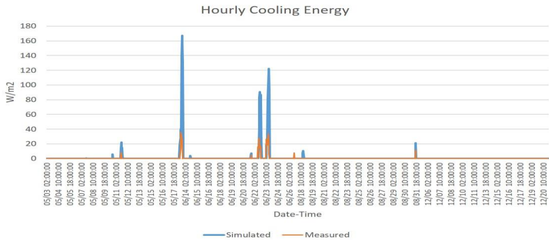
Figure 10. Hourly cooling energy comparison between simulation and measurement.
