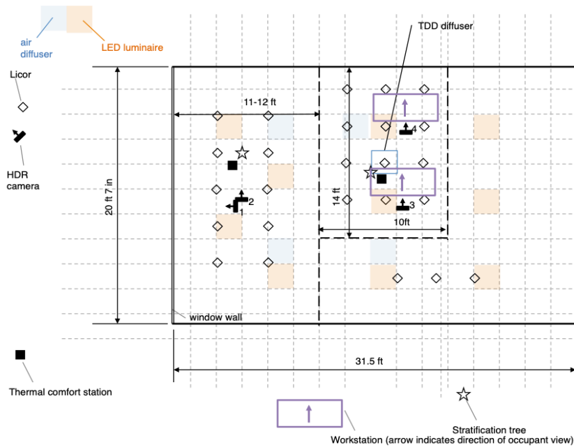
Figure 5. Test cell configuration for the ZNE package tests. Test cell (Cell B) is shown. Baseline cell (Cell A) configuration was similar except a) the size and location of luminaires was different (nine 2 x 4 ft fluorescent troffers instead of ten 2 x 2 ft LED luminaires) and b) the cell was symmetrical along the horizontal axis of this figure.
