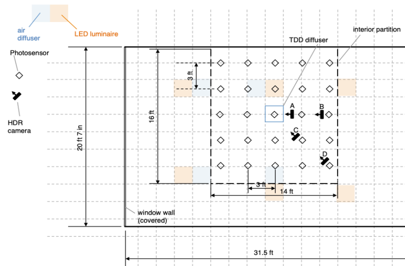
Figure 6. Test cell configuration for the TDD tests. Position of luminaires is shown but luminaires were not powered during these tests.
