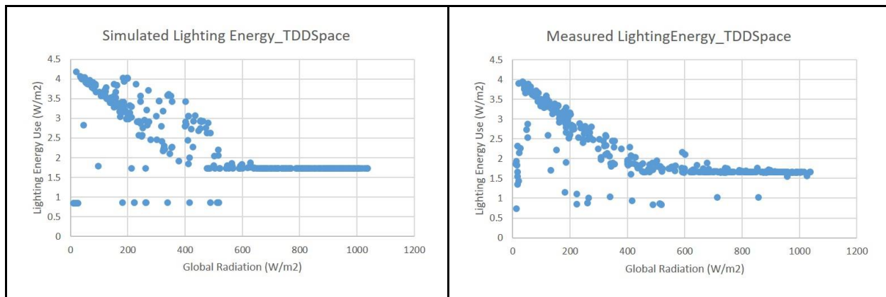
Figure 8. Variation of the TDD space lighting energy use with global radiation - simulated vs. measured.
