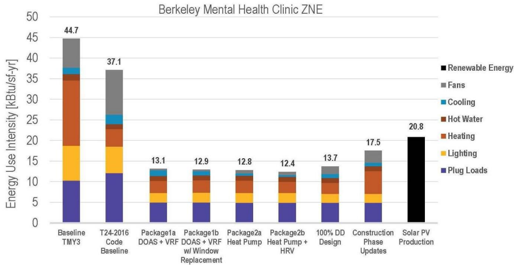
Figure 16. Site Demonstration Site Simulation Analysis of Several ZNE Packages and Comparison with Title 24 Energy Code and On-Site PV Production
