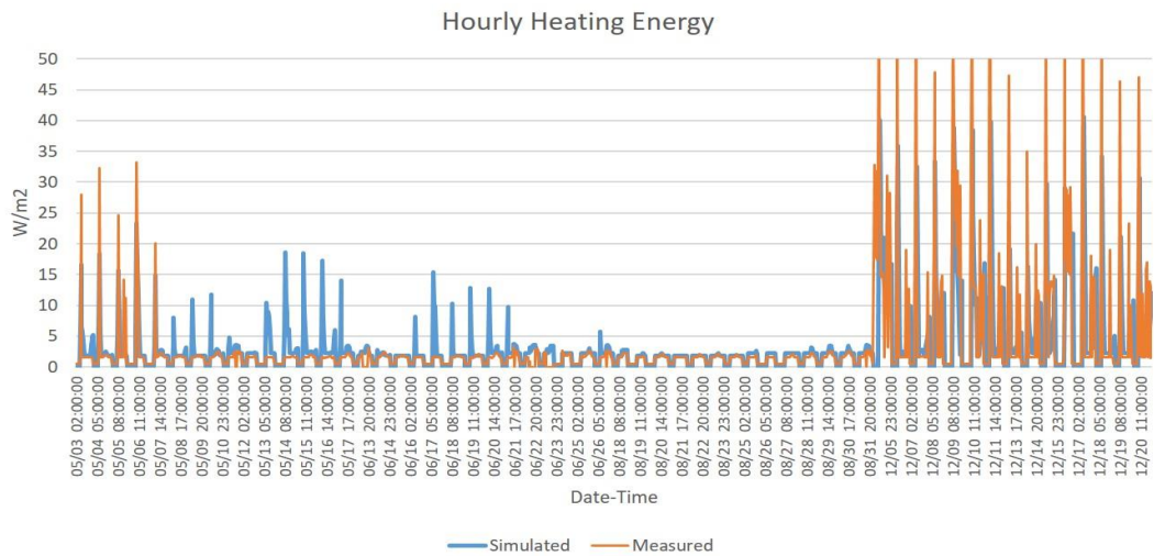
Figure 11. Hourly heating energy comparison between simulation and measurement.
