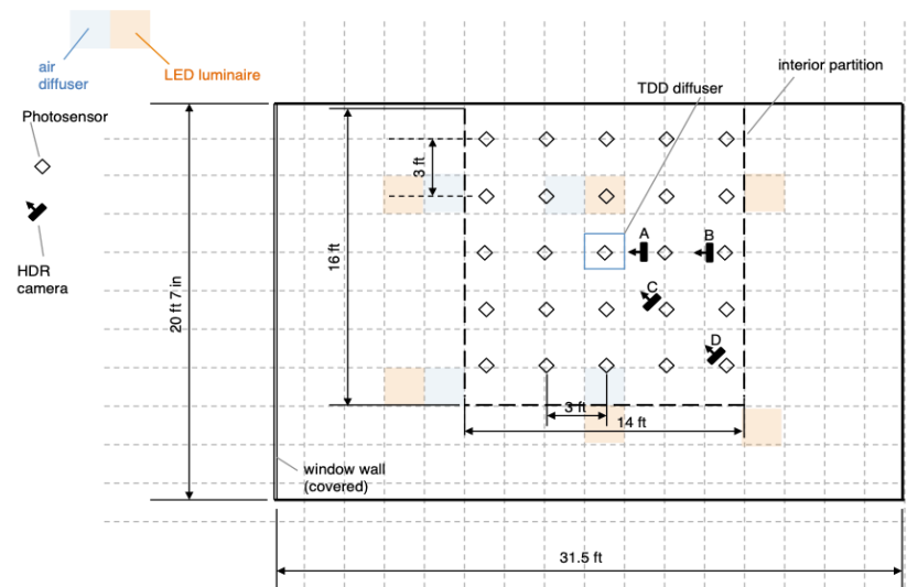
Figure 6. Test cell configuration for the TDD tests. Position of luminaires is shown but luminaires were not powered during these tests.
