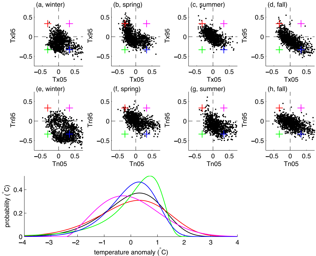
FIG. 6. Mean-T05 slopes vs mean-T95 slopes for each season and for (a)–(d) Tx and (e)–(h) Tn. Dashed lines demarcate quadrants that, moving from top right counterclockwise, indicate that mean warming is associated with more positive skew, greater variance, more negative skew, and less variance. U.S. stations are generally aligned along the axis of more or less variance. At bottom is a generalized extreme value probability distribution (black) with coefficients chosen to be approximately consistent with average summer Tx. The distribution has its orientation reversed from the usual definition such that it has negative skew. Also plotted are alterations of the base distribution that have values of T05 and T95 values consistent with a 1°C mean warming for the various mean-extreme slopes indicated by the colored crosses in the scatterplots. The red distribution, for example, has a 0.67°C increase in spread between the 5th and 95th percentiles. To aid in visual comparison, all distributions are centered on zero.
