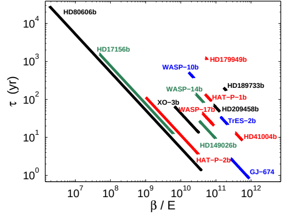
Figure 8: (Colour online) Typical (inviscid) growth time \tau of the elliptical instability in the hot Jupiter vs. the control parameter \beta/E (see eq. 1), assuming a molecular kinematic viscosity \nu = 10^{-6} \text{ m}^2 \text{ s}^{-1} (Zhang and Schubert 1996).
