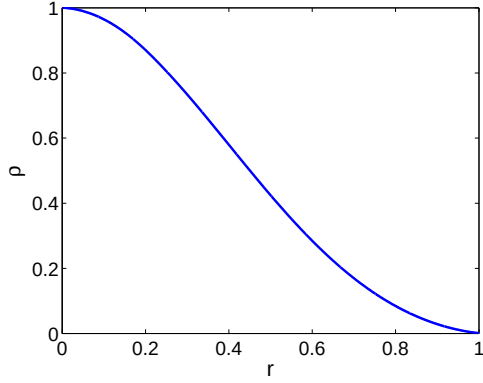
Figure 6: Density profile imposed at each time step along ellipsoids homothetic to the surface r = \sqrt{(x/a)^2 + (y/b)^2 + (z/c)^2} = 1 .
