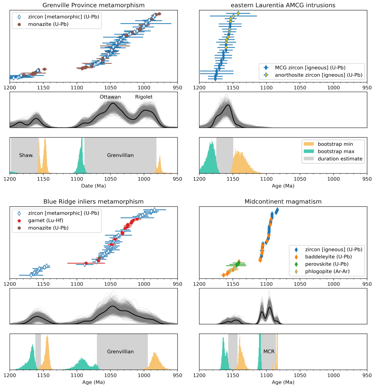
Figure 2: Compilation of geochronological data that provide insight into late Mesoproterozoic tectonics within Laurentia. The top panels in each group show the dates with their 2\sigma uncertainties keyed by mineral and method. The middle panel shows the kernel density estimates (continuous probability density estimate curves) for the dates in black and for bootstrap/Monte Carlo resamples of the data using the methods described in the text. The lower panel shows histograms of the maximum and minimum bounds from these distributions. The grey boxes provide estimates of the duration of the event constrained by the geochronology and robust to the resampling approach providing likely durations. These durations are: Shawinigan orogeny, Grenville Province 1198 to 1157 Ma; Grenvillian orogeny, Grenville Province 1089 to 981 Ma; pre-Grenvillian orogeny, Blue Ridge 1162 to 1153 Ma; Grenvillian orogeny, Blue Ridge 1070 to 994 Ma; AMCG plutonism 1174 to 1149 Ma; pre-Midcontinent Rift magmatism 1157 to 1143 Ma; Midcontinent Rift magmatism 1108 to 1086 Ma. The data come from the Canadian Geochronology Knowledgebase compilation (2013) as well as additional data sets compiled in this work from the following publications: Aleinikoff et al. (2013, 2021), Bleeker et al. (2020), Chiarenzelli et al. (2011), Connelly (2006), Davis and Green (1997a), Dunning and Indares (2010), Fairchild et al. (2017), Hamilton et al. (2004), Jannin et al. (2018a, 2018b), Johnson et al. (2018, 2020), Jordan et al. (2006), Krogh et al. (1987), Labat et al. (2020), Lasalle et al. (2014), Markley et al. (2018), McCormick et al. (2017), McLelland et al., (2004), Moecher et al. (2020), Paces and Miller (1993), Peck et al. (2018), Queen et al. (1996), Regan et al., (2019), Shinevar et al. (2021), Smith et al. (2020), Southworth et al. (2010), Swanson-Hysell et al. (2019, 2021b), Tollo et al. (2010, 2017), Williams et al., (2019), Wu et al. (2017). For some data sets, new weighted means were calculated for populations of dates. The data compilation as well as the Python code used for the analysis are available in a Github repository: https://github.com/Swanson-Hysell/Mesoproterozoic_Turning_Point and in this Zenodo archive: https://doi.org/10.5281/zenodo.7098504 .
