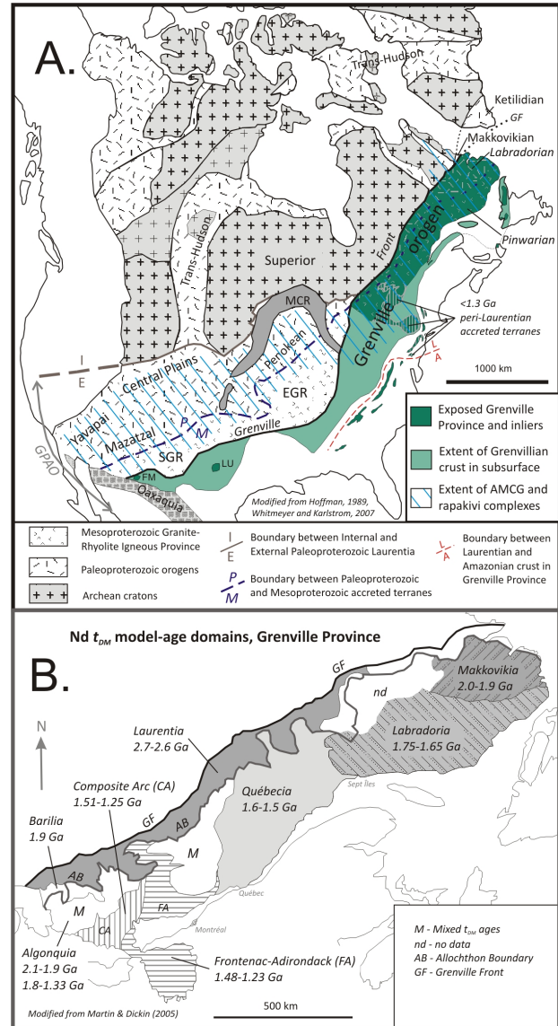
Figure 1: (A): Precambrian tectonic provinces of Laurentia, illustrating the trajectory of the Grenville Front cutting obliquely across External Laurentia in the subsurface and intersecting the boundary with Internal Laurentia in the western Grenville Province. Abbreviations: EGR, SGR, Mesoproterozoic Eastern and Southern Granite-Rhyolite provinces; GF, Grenville Front; GPAO, Great Proterozoic Accretionary Orogen; MCR, Midcontinent Rift. The Labrador Orogen (age-equivalent to the Mazatzal Orogen) and Pinwarian Orogen (in part age-equivalent to the EGR), are reworked parts of the Great Proterozoic Accretionary Orogen within the Grenville Orogen. The extent of AMCG and rapakivi suites in southwestern Laurentia is after McLelland et al., 2010b). The boundary between Laurentian and allochthonous lithosphere (potentially derived from Amazonia; L/A) is based on whole-rock Pb isotope data. FM, Franklin Mountains; LU - Llano Uplift. Oaxaquia is a separate Rodinia fragment accreted to Laurentia in the Mesozoic (modified from Rivers et al., 2012; after Hoffman, 1989; Loewy et al., 2004; Whitmeyer and Karlstrom, 2007, where references to original sources are provided). (B) Map showing depleted mantle Nd model age (Nd t_{DM} ) domains of the Grenville Province (modified from Rivers et al., 2012, after Martin and Dickin, 2005).
