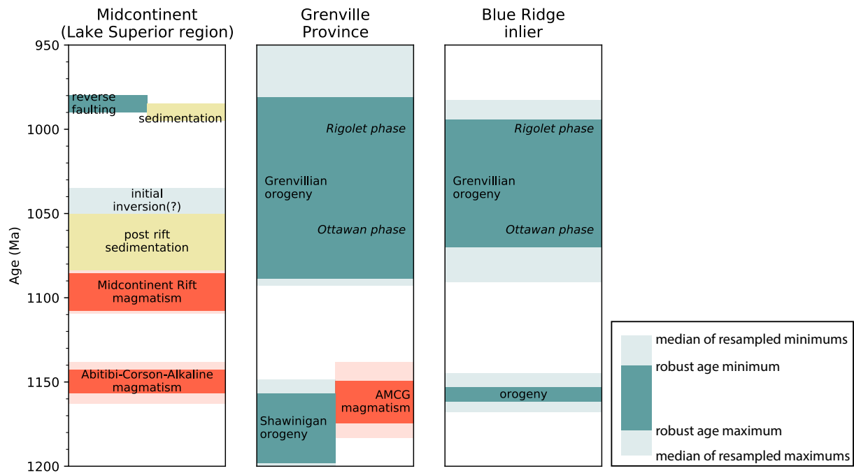
Figure 3: Simple timelines of tectonic and tectonomagmatic events in the Midcontinent-Lake Superior region, the Grenville Province, and the Mesoproterozoic Blue Ridge inlier. The times shown for orogenic events and for magmatic events are directly taken from the analysis of the geochronology data in Figure 2 with additional constraints for sedimentation in the Midcontinent as described in the text. The darker colors represent the bounds on the 5th percentile of the resampled maximum ages and the 95th percentile of the resampled minimum ages. This range, which is more robust to resampling, is interpreted to constrain the duration of the magmatic or orogenic interval. The fainter colors are the medians of those bounds, indicating that there are dates that imply those ages, but they are more likely to be outliers due to low precision. This compilation highlights AMCG magmatic activity being a late to post-Shawinigan phenomenon and temporally overlapping with magmatic activity in the Midcontinent. Note that the onset of Grenvillian collision orogenesis is closely temporally related to the end of Midcontinent Rift magmatism, which itself is closely associated with the end of extension.
