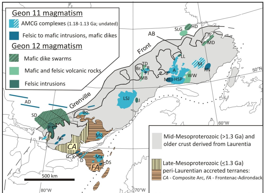
Figure 4: Sketch map of the Grenville Province and its immediate foreland, showing the Allochthon Boundary (AB), late Mesoproterozoic (<1.3 Ga) pericratonic accreted terranes, and major magmatic units emplaced during geons 12 and 11 (a geon is a 100 million year interval ; Hofmann 1990; for instance geon 12 is all ages between 1200 and 1299.9 Ma). Abbreviations: A, Atikonak-Lac Fournier anorthosite massif; AD, Abitibi dikes; AG, Algonquin gabbros; B, Baune gabbro; Bo, Bouchette anorthosite; Br, Brien anorthosite; D, Diana AMCG complex; DS, Dresden Station gabbro; FT, Fe-Ti gabbro; G, Gananoque monzogranite suite; J, Joncas mangerite; HD, Harp dikes; HSP - Havre St-Pierre anorthosite massif; K, Kingston dikes; LBS, Layered bimodal sequence; LSJ, Lac St-Jean anorthosite massif; LL, Lac Long tonalite; M, Mécatina anorthosite massif (undated); Ma, Marcy, Snowy Mountain and Oregon Dome anorthosite massifs, spatially associated syenite, monzonite, granite; MB, Manicouagan extensional belt; Mo, Morin anorthosite massif; MD, Mealy dikes; Mt, Manitou monzonite-diorite-granite complex; P, includes Powassan, Sturgeon Falls, Mulock and Bonfield monzogranitic plutons, St-Charles and Mercer anorthosites; PI, Parry Island anorthosite; R, Rodot anorthosite-leucogabbro; RN, Robe noire mafic sills; SD, Sudbury dikes, SLG, Seal Lake Group; TD, Touloustouk dikes; WW, rhyolite in western Wakeham domain. Modified after Rivers et al. (2012), with additional information from Indares and Moukhsil (2013), where ages and original references are given.
