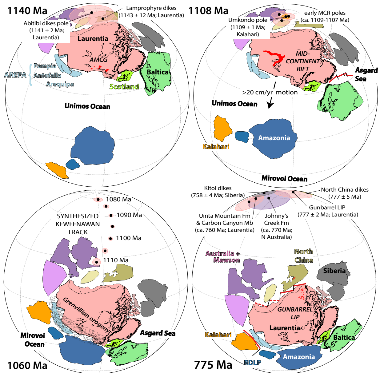
Figure 5: Paleogeographic reconstruction of Laurentia and adjacent Proterozoic continents in the late Mesoproterozoic and early Neoproterozoic at different time slices. Laurentia's position is constrained by paleomagnetic poles shown on the reconstructions. In the 1140 Ma time slice, the ca. 1170 to 1150 Ma AMCG complexes are shown (red). Baltica is shown in the northern Europe and North America (NENA) configuration which is supported paleomagnetically from 1750 to at least 1270 Ma and potentially to 1122 Ma (Evans and Pisarevsky, 2008; Salminen et al., 2009; Swanson-Hysell et al., 2021a) before rifting away from East Greenland to open the Asgard Sea (Cawood et al., 2010; Cawood and Pisarevsky, 2017). The AREquipa-Pampia-Antofalla (AREPA) ribbon continent (see discussion in Macdonald et al., this volume) arrived prior to or during the Grenvillian orogeny and may have collided ca. 1140 Ma as shown, resulting in the Llano orogeny and orogenesis recorded in the Blue Ridge inliers. Paleomagnetic poles constrain Amazonia and Kalahari to have been separate from Laurentia prior to the Grenvillian orogeny when they could have been on a conjugate plate. At 1108 Ma during the early plateau phase of the Midcontinent Rift when Laurentia was at high latitudes, the Kalahari craton is constrained to have been straddling the equator by paleomagnetic data from the Umkondo large igneous province (Swanson-Hysell et al., 2015). A synthesis of the Keweenaw Track resulting from an Euler pole inversion (Swanson-Hysell et al., 2019) is shown in the 1060 Ma timeslice. This path records the rapid motion of Laurentia towards the equator between ca. 1108 and 1080 Ma during the time period when the Unimos Ocean was being consumed prior to the collisional orogenesis associated with the Grenvillian orogeny. The assembled Rodinia persisted until initial rifting ca. 775 Ma with episodic rifting continuing until ca. 530 Ma. This history is summarized in Figure 3 of Macdonald et al. (this volume). The code and Euler pole parameters used to generate this model are available here: https://github.com/Swanson-Hysell1/Mesoproterozoic_Turning_Point
