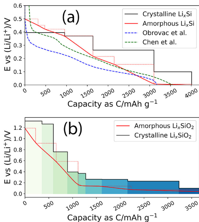
Fig. 5. Calculated electrode potential profile ( E vs (\text{Li}/\text{Li}^+)/\text{V} ) for crystalline and amorphous a) lithium silicides in comparison with experimental curves [18,89] and b) lithium silicates. The dashed red line in both a) and b) corresponds to the voltage of the amorphous phases as calculated from the convex hull before smoothing. (For interpretation of the references to color in this figure legend, the reader is referred to the Web version of this article.)
