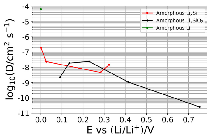
Fig. 6. Room temperature Li self-diffusion coefficients in amorphous lithium silicides and lithium silicates as a function of electrode potential E vs (\text{Li}/\text{Li}^+)/\text{V} .
