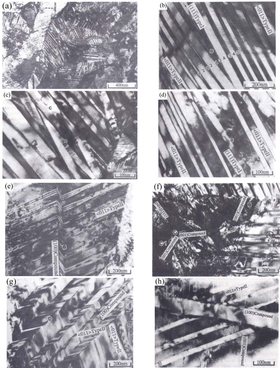
Figure 2.19 Various twins observed in B19' martensite upon transformation from B2 – B19' [168, 169].
