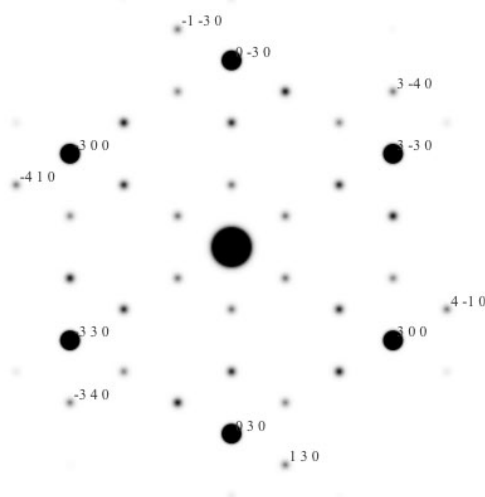
Figure 2.34 Simulated electron diffraction pattern of R-phase (space group P\bar{3} ). Pattern indexing is with respect to \langle 001 \rangle zone. The pattern is calculated using Crystal Maker's Single Crystal software program. Compare the pattern with that of Hara reproduced in [47].
