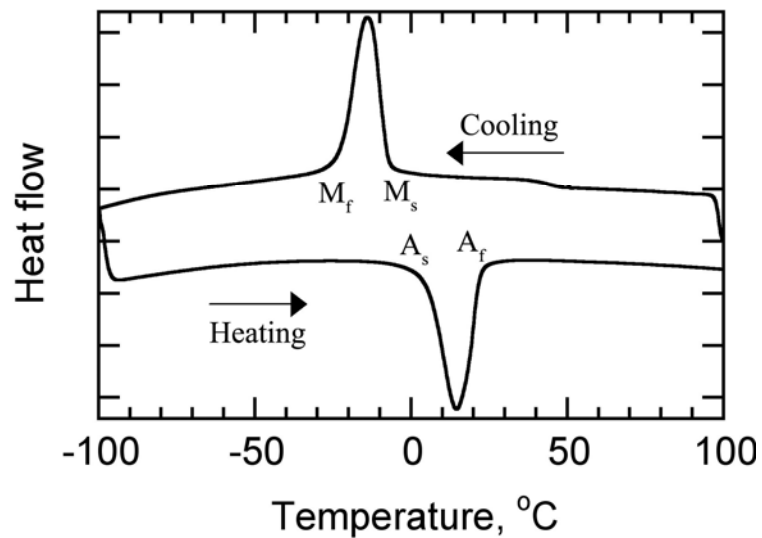
Figure 2.8 DSC trace of fully annealed ( 800^{\circ}\text{C} , 0.5-hr) 50.8-NiTi and the corresponding transformation temperatures, M_s , M_f , A_s and A_f .
