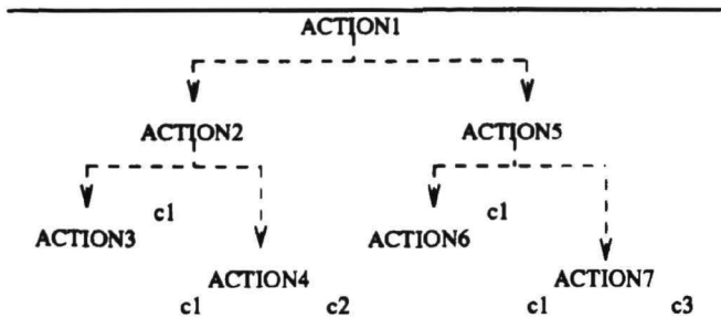
Figure 1: Schematic Discourse Plan Illustrating a Redundant Step
