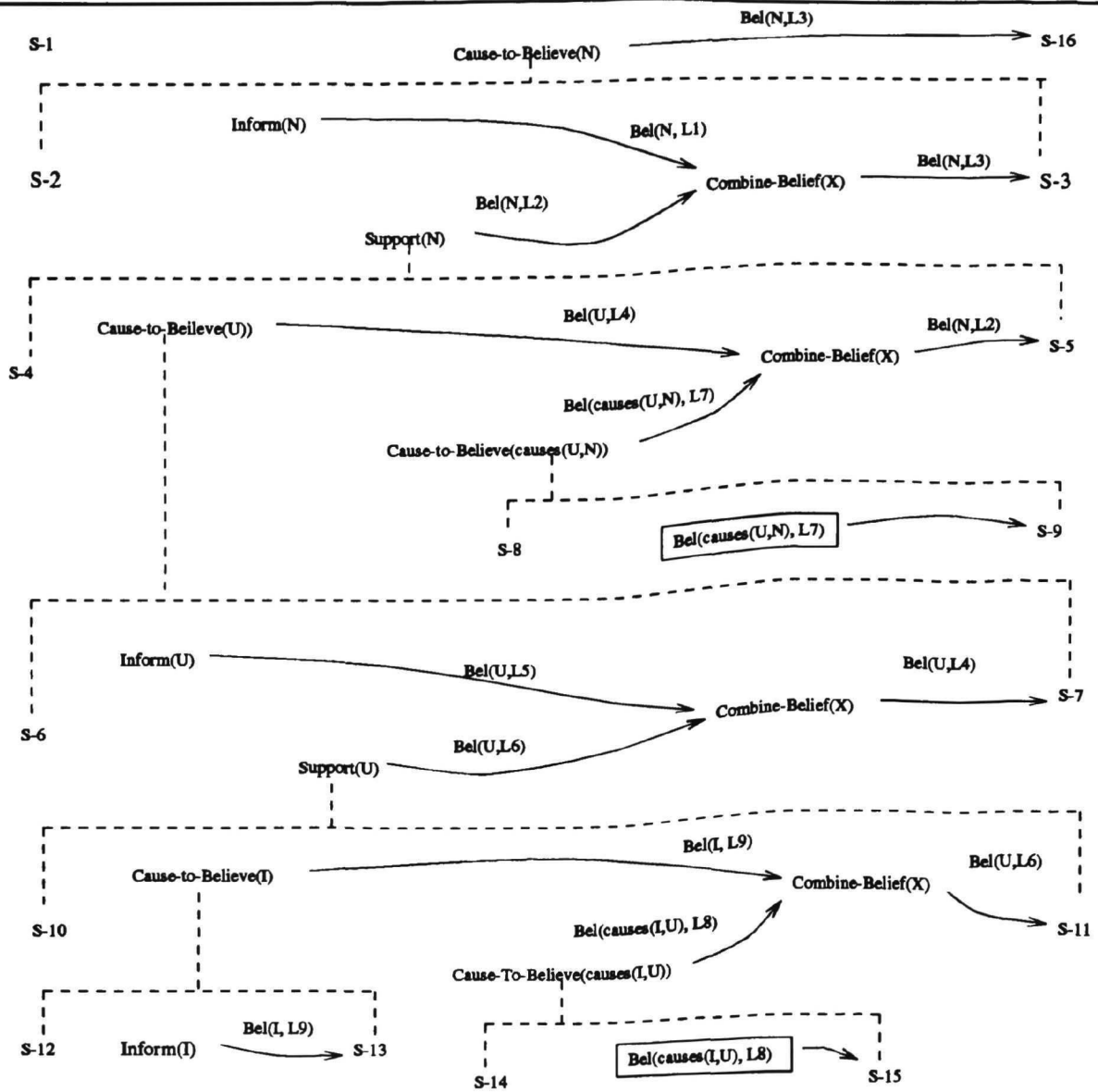
Figure 3: An Example Discourse Plan
