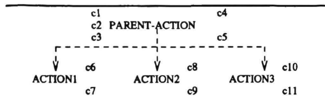
Figure 1: Schematic Discourse Plan Illustrating a Redundant Step
