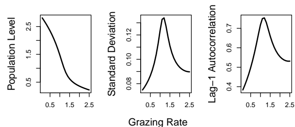
Figure 3: A system where critical slowing down is observed without a critical threshold, from KÄlfi et al. (2012). In this model, prey have logistic growth and are subject to predation with a Type III functional response, but there is no bifurcation. Instead, average prey population exhibits a smooth response to increased predation (grazing). Left: The population level as a function of predation rate. Middle: Variance of the prey population level. Right: Lag-1 Autocorrelation in prey population dynamics as grazing rate increases. Note that both indicators increase despite the lack of a bifurcation.
