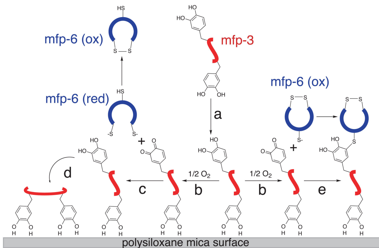
Figure 3. Redox control and the stepwise adsorption and cross-linking of mfp-3
