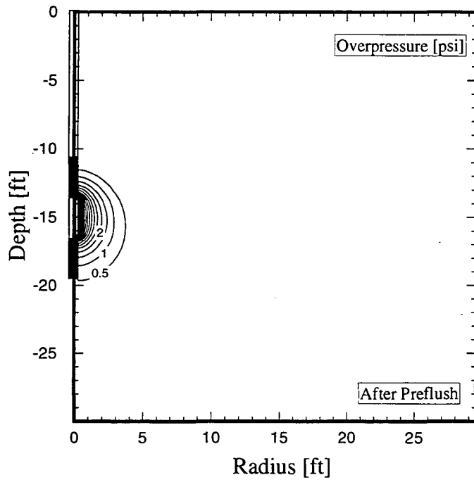
Figure 17: Liquid saturation and pressure distribution after preflushing
