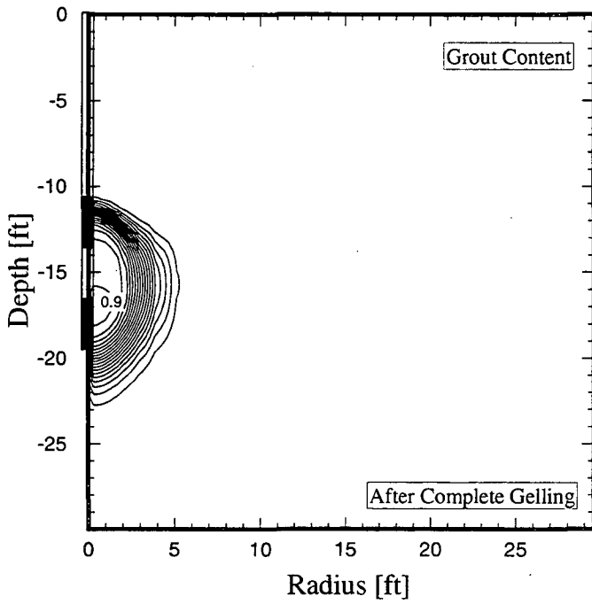
Figure 21: Liquid saturation and grout content at the end of the gelling period
