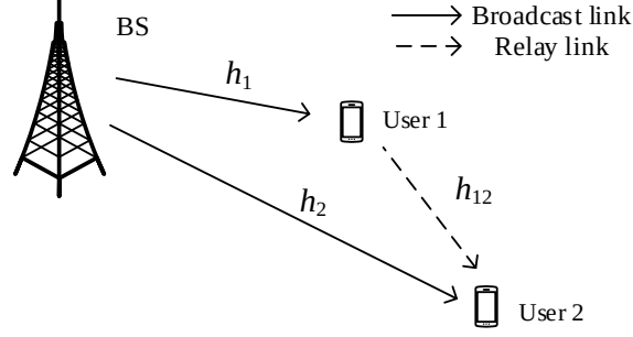
Fig. 1: Illustration of a three-node C-ANOMA/C-NOMA system with user relaying.
