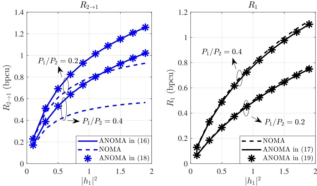
Fig. 4: The throughputs R_{2 \rightarrow 1} and R_1 as functions of the channel gain |h_1|^2 for C-ANOMA and C-NOMA systems when N = 10 , \tau = 0.5 , P_1 + P_2 = 5 .
