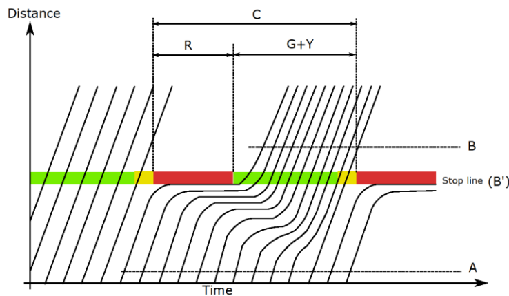
Figure 2. Distance-time diagram for a signalized intersection.
