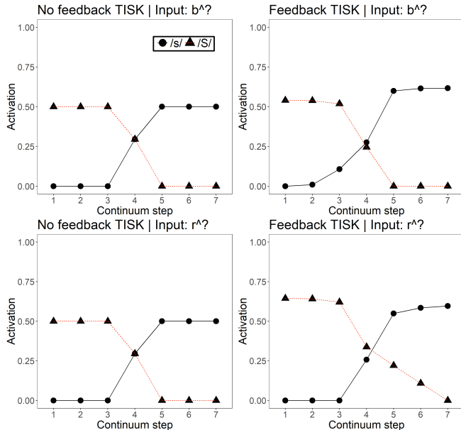
Figure 6: Lexical effects on phoneme activations. Top: input is b^? , where /? is a continuum between /s/ and /ʃ/ . On the left is the result with TISK without feedback, with activations plotted for /s/ and /ʃ/ ; activations change approximately linearly across the continuum. On the right, results are plotted with TISKfb; crucially, activations of /s/ increase, as they are consistent with the lexical item bus , while no changes is seen for /ʃ/ , which corresponds to a nonword ending with sh but the same onset as bus . On the bottom row, the opposite pattern is observed, as /ʃ/ is consistent with the word rush , while /s/ would make the nonword *russ .
