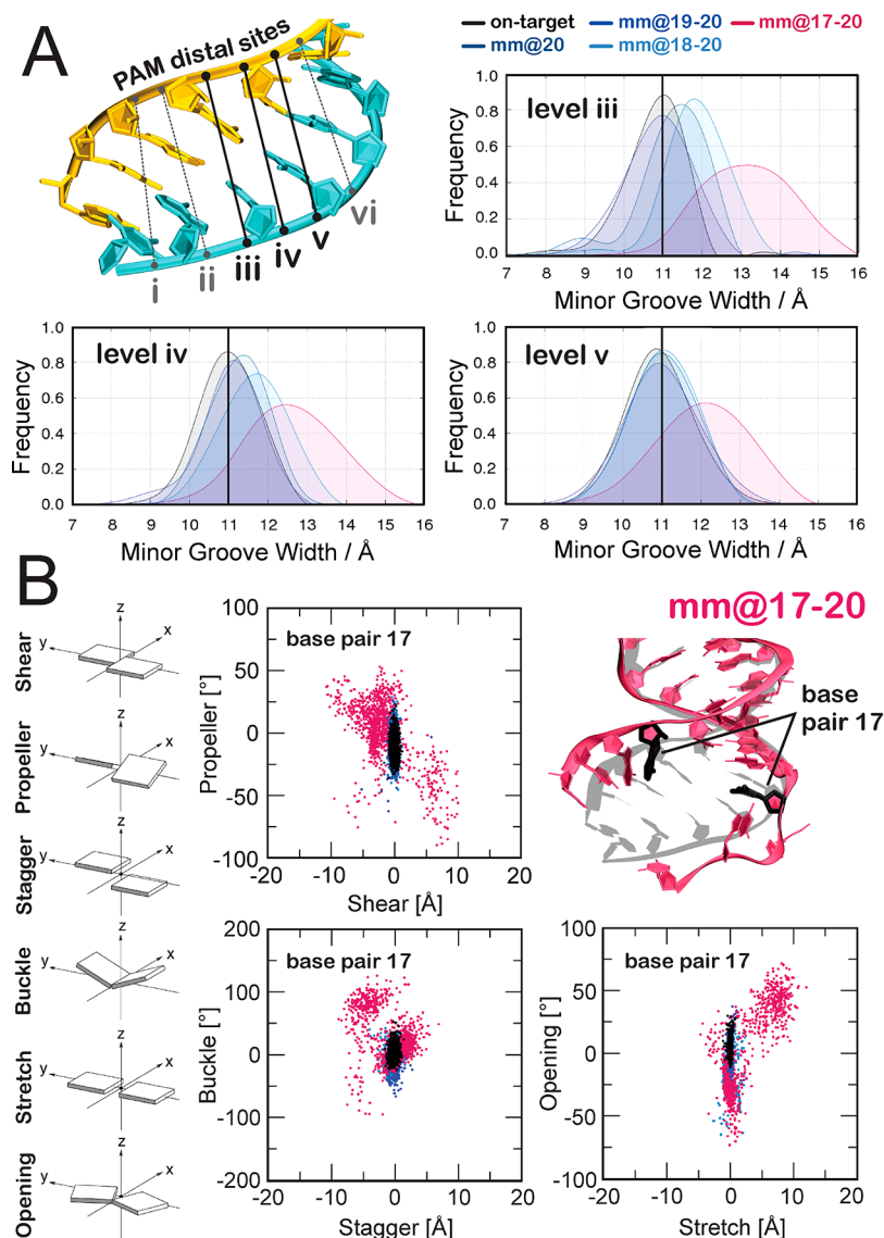
Figure 3. RNA:DNA geometrical properties along GaMD simulations. (A) The RNA:DNA minor groove width has been computed in the PAM distal region at six different levels (i–vi, from positions 20 to 16 of the TS), which are schematically shown on the 3D structure of the RNA:DNA hybrid. The probability distributions of the RNA:DNA minor groove width at the iii–v levels are shown for the on-target CRISPR-Cas9 and for the systems including base pair mismatches at different positions of the hybrid (i.e., mm@20, mm@19–20, mm@18–20, and mm@17–20). A vertical bar indicates the experimental minor groove width (i.e., ~11 Å from X-ray crystallography, enlarged by ~1 Å if NMR data are considered). 29 Full data are reported in Figure S2. (B) Scatter plots of the geometrical base pair descriptors, computed at position 17 of the RNA:DNA hybrid for all studied systems (full data are in Figures S3–S5). Translational (i.e., shear, stretch, and stagger) and angular (i.e., buckle, propeller, and opening) descriptors are expressed in Å and degrees, respectively. The RNA:DNA hybrid is shown on the right for the on-target CRISPR-Cas9 (gray) superposed to the mm@17–20 (red) system.
