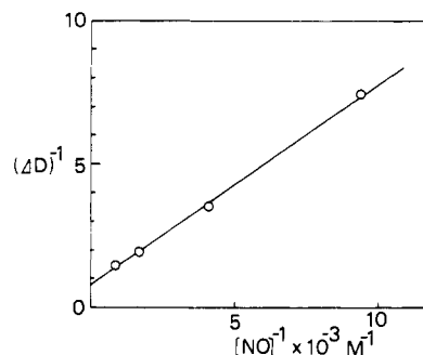
Figure 2. Plot of (\Delta D)^{-1} at 393 nm vs [\text{NO}]^{-1} for determination of the equilibrium constant for \text{Fe}^{\text{III}}\text{TPPS} + \text{NO} \rightleftharpoons (\text{NO})\text{Fe}^{\text{III}}\text{TPPS} .
