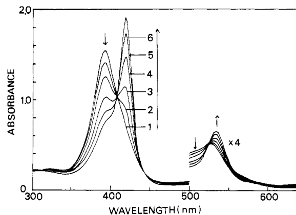
Figure 1. Absorption spectral changes of 1.0 \times 10^{-5} \text{ M} \text{Fe}^{\text{III}}\text{TPPS} in an aqueous solution in the presence of NO: 1, [\text{NO}] = 0 \text{ M} ; 2, [\text{NO}] = 1.06 \times 10^{-4} \text{ M} ; 3, [\text{NO}] = 2.43 \times 10^{-4} \text{ M} ; 4, [\text{NO}] = 6.0 \times 10^{-4} \text{ M} ; 5, [\text{NO}] = 1.15 \times 10^{-3} \text{ M} ; 6, [\text{NO}] = 1.43 \times 10^{-3} \text{ M} .
