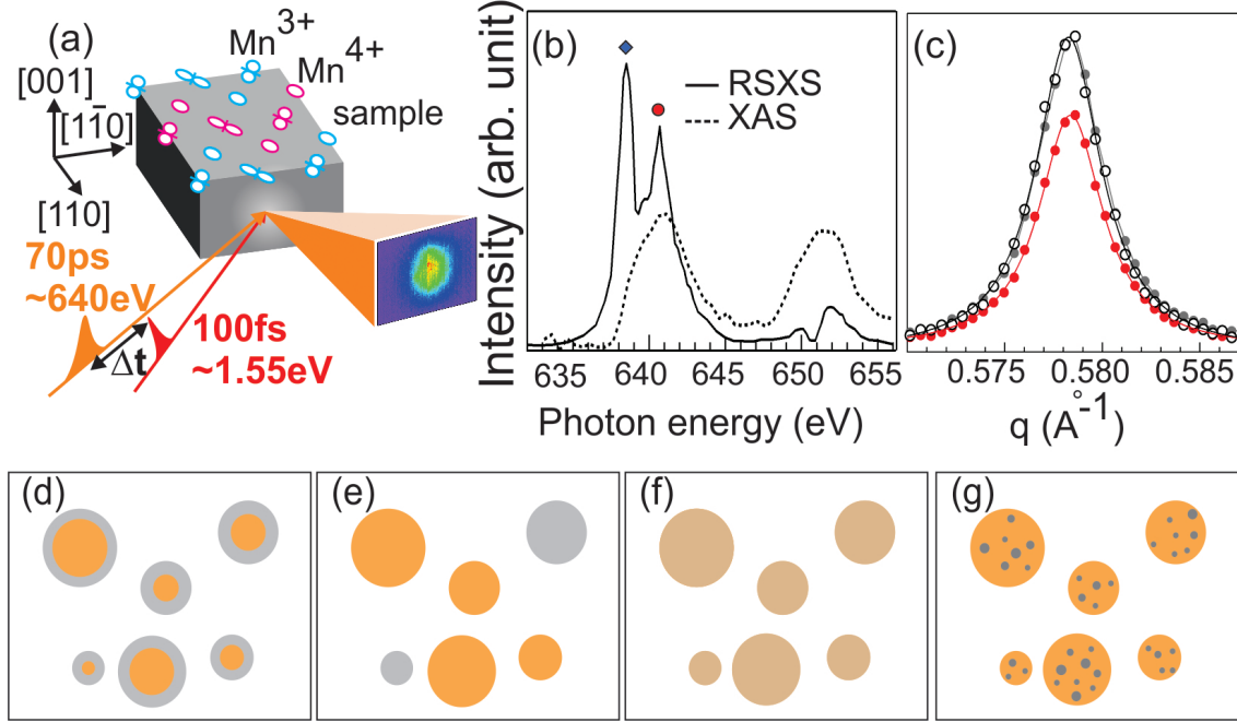
FIG. 1: (a) Schematic diagram of the CE-type SO state overlaid with the experimental geometry for TR-RSXS measurements. Circles and lobes represent the \text{Mn}^{4+} sites and e_g orbitals of the \text{Mn}^{3+} sites. Pink and blue colors represent opposite spin orientations. (b) Energy profile of the SO diffraction peak from static RSXS measurements (solid line) as compared to the XAS spectrum (dotted line). The symbols mark the photon energies used in the time-resolved measurements. (c) Comparison of the SO diffraction peak intensity measured at 641.4 eV before (open circles) and \Delta t=500 ps after 800 nm laser excitation at 1 \text{ mJ}/\text{cm}^2 pump fluence (red filled circles). Solid lines are fits using a Lorentzian function. Gray filled circles are data taken at \Delta t=500 ps rescaled by a factor of 1.33. (d-g) Schematic illustrations of four different responses of SO domains to photo-excitation. The orange areas represent the SO domains and the gray areas represent the regions destroyed by photo-excitation. These are over-simplified models and a realistic picture is likely more complicated due to the irregular shapes and interconnections between SO domains.
