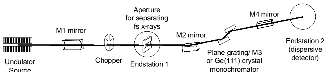
Figure 22. Schematic layout of beamline 6.0.1.
