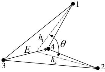
Figure 5: The bending angle and its neighboring triangles.
