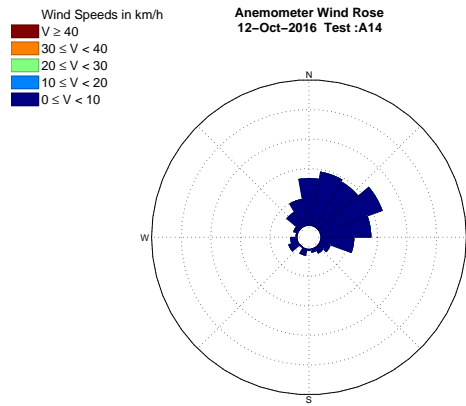
Figure B.25: Wind Rose - 12 October 2016 Test A1.4
