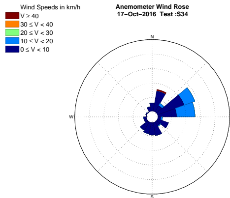
Figure B.38: Wind Rose - 17 October 2016 Test S3.4
