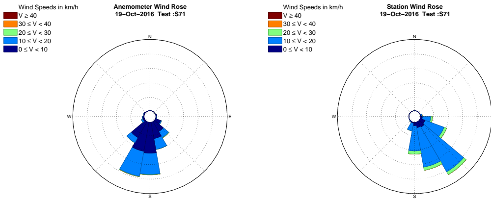
Figure B.45: Wind Rose - 19 October 2016 Test S7.1
