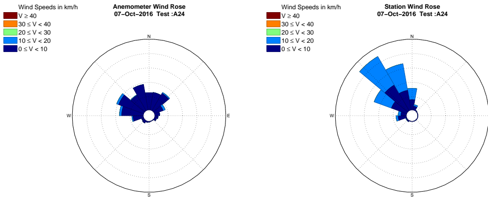
Figure B.11: Wind Rose - 7 October 2016 Test A2.4
