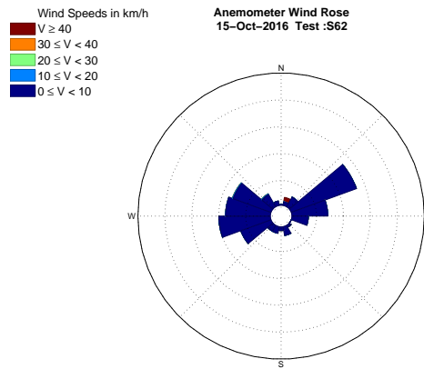
Figure B.30: Wind Rose - 15 October 2016 Test S6.2
