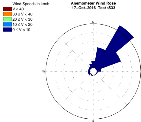
Figure B.37: Wind Rose - 17 October 2016 Test S3.3
