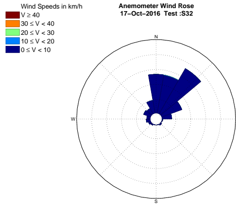
Figure B.36: Wind Rose - 17 October 2016 Test S3.2
