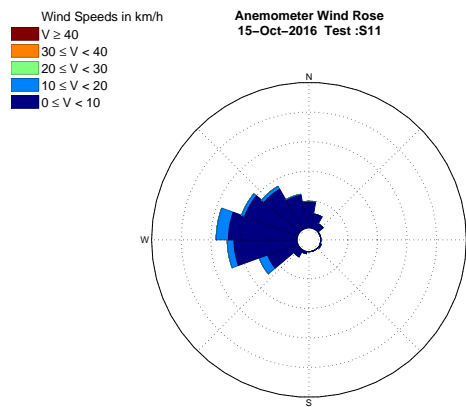
Figure B.26: Wind Rose - 15 October 2016 Test S1.1
