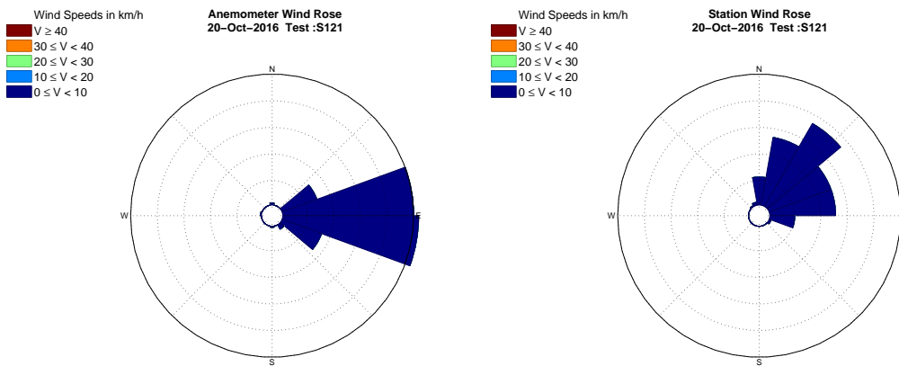
Figure B.47: Wind Rose - 20 October 2016 Test C1.1
