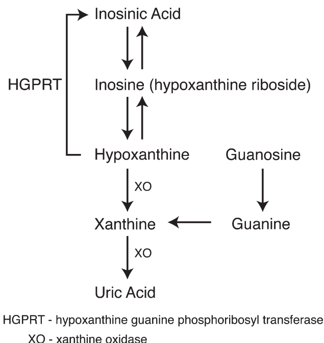
Fig. 3. Uric acid metabolism.
