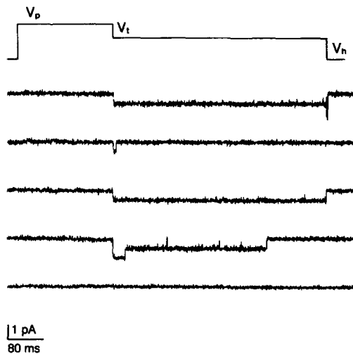
FIGURE 1. Unitary Ba 2+ currents recorded from cell-attached patches on the surface membrane of C2 myotubes. Channel openings were evoked by the pulse paradigm shown at the top of the figure. The patch was depolarized from a holding potential of -70 to +50 mV for ~224 ms after which the potential was stepped down to -10 mV for ~500 ms before returning to the holding potential. Records were corrected for linear leak and capacity currents as described in Materials and Methods. The cell was bathed in an isotonic K + asparate solution to zero the cell's resting potential. The patch electrode contained 110 mM BaCl 2
