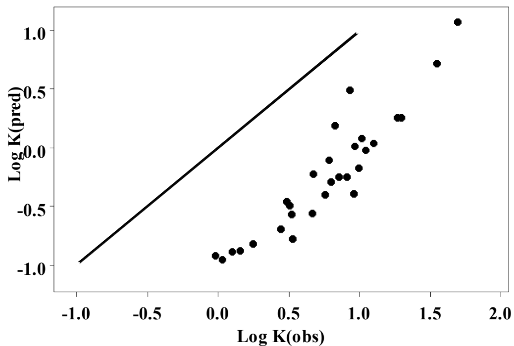
FIGURE 1. A plot of \log K for 1:1 association in octan-1-ol predicted on eq 8, against observed values of \log K , from Table 3; the line is that of unit slope.
