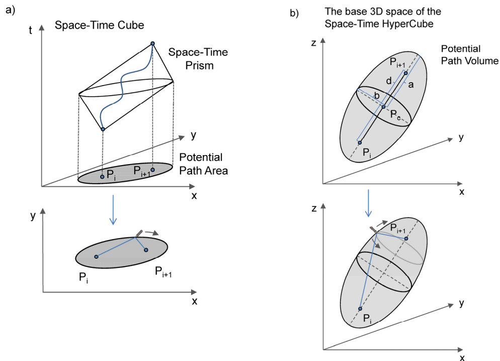
Figure 1: a) The definition of the Potential Path Area as the projection of the Space-Time Prism in an STC and b) its 4D generalisation the Potential Path Volume.
