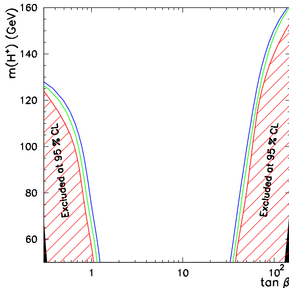
Figure 5: D0 search for charged Higgs bosons in top decays [10]. The hatched regions of scalar mass and \tan\beta are excluded.
