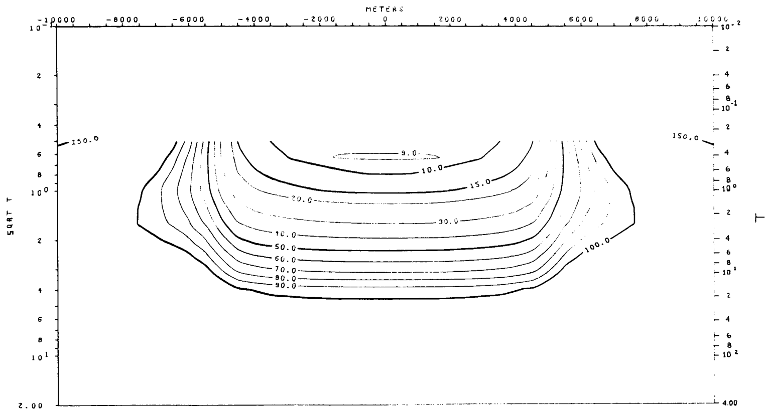
TE MODE APPARENT RESISTIVITY VS. PERIOD (T) MODEL 4-b
