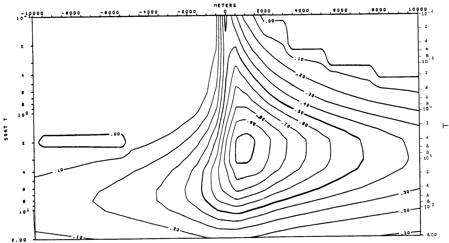
TIPPER VS. PERIOD (T) MODEL 6-c
