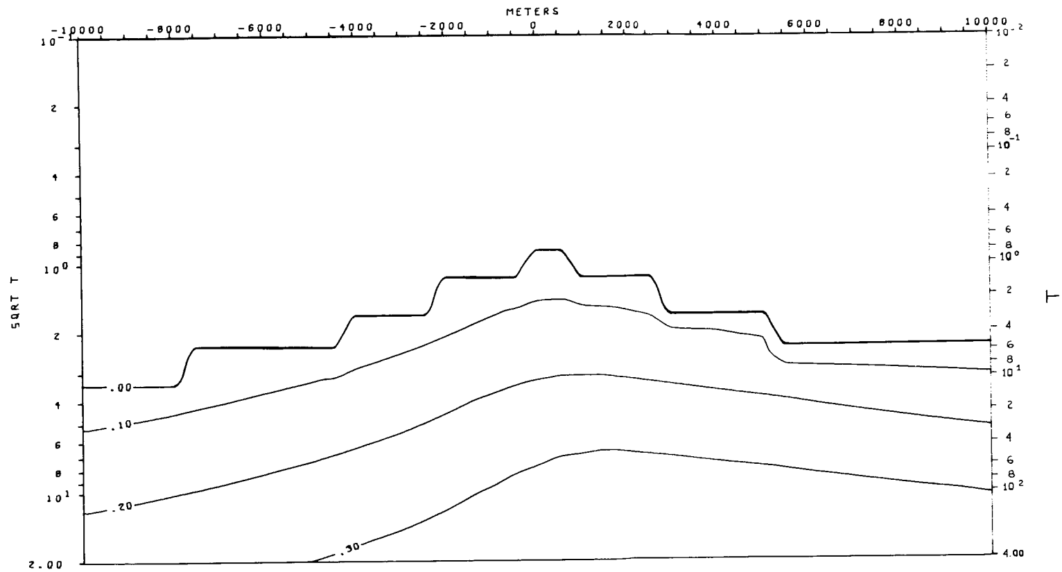
TIPPER VS. PERIOD (T) MODEL 3-b
