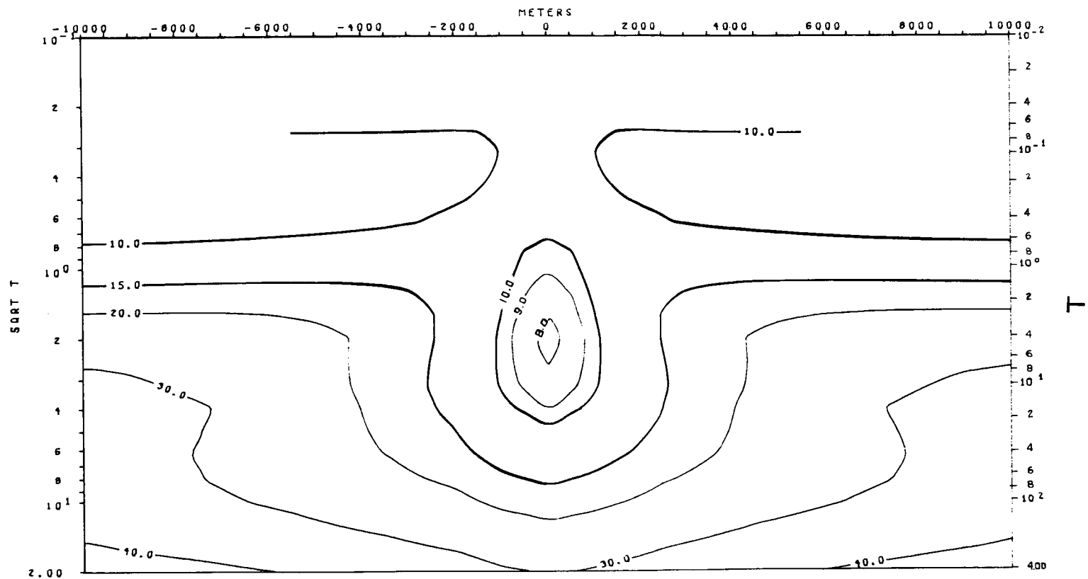
TE MODE APPARENT RESISTIVITY VS. PERIOD (T) MODEL 5-a
