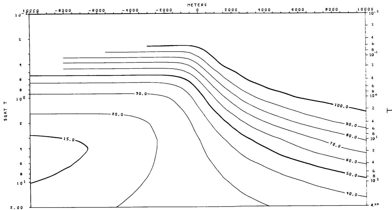
TE MODE APPARENT RESISTIVITY VS. PERIOD (T) MODEL 3-c
