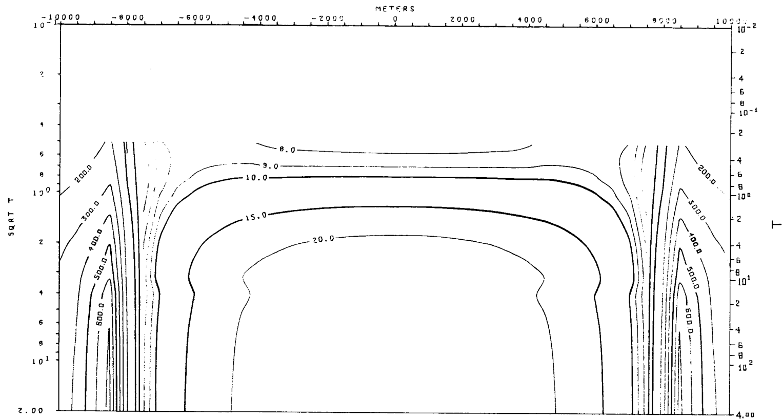
TM MODE APPARENT RESISTIVITY VS. PERIOD (T) MODEL 4-c
