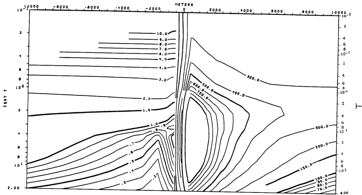
TM MODE APPARENT RESISTIVITY VS. PERIOD (T) MODEL 6-c
