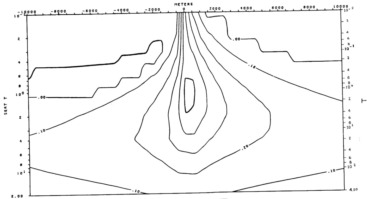
TIPPER VS. PERIOD (T) MODEL 4-d
