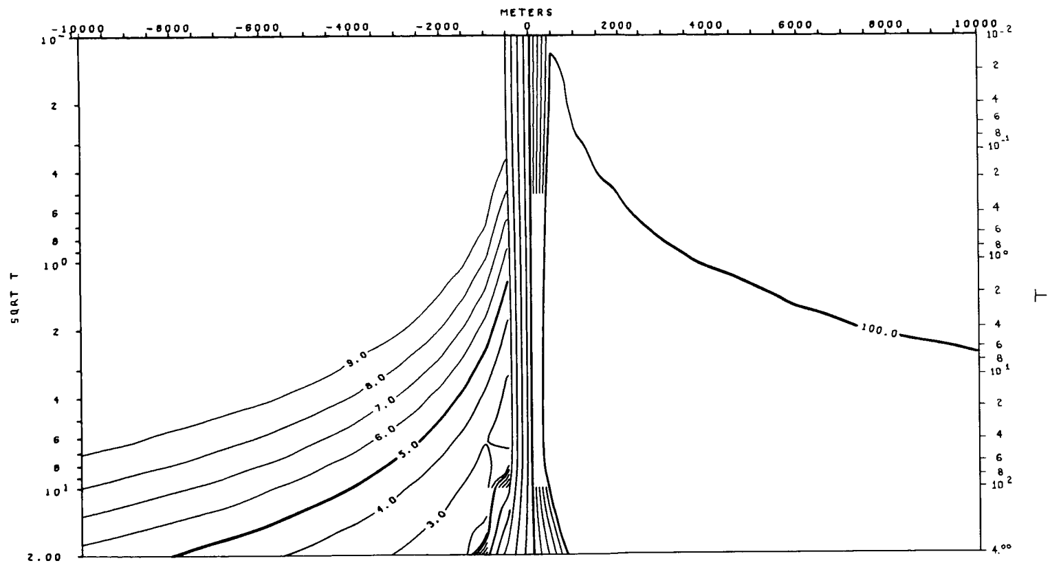
TE MODE APPARENT RESISTIVITY VS. PERIOD (T) MODEL 1-c
