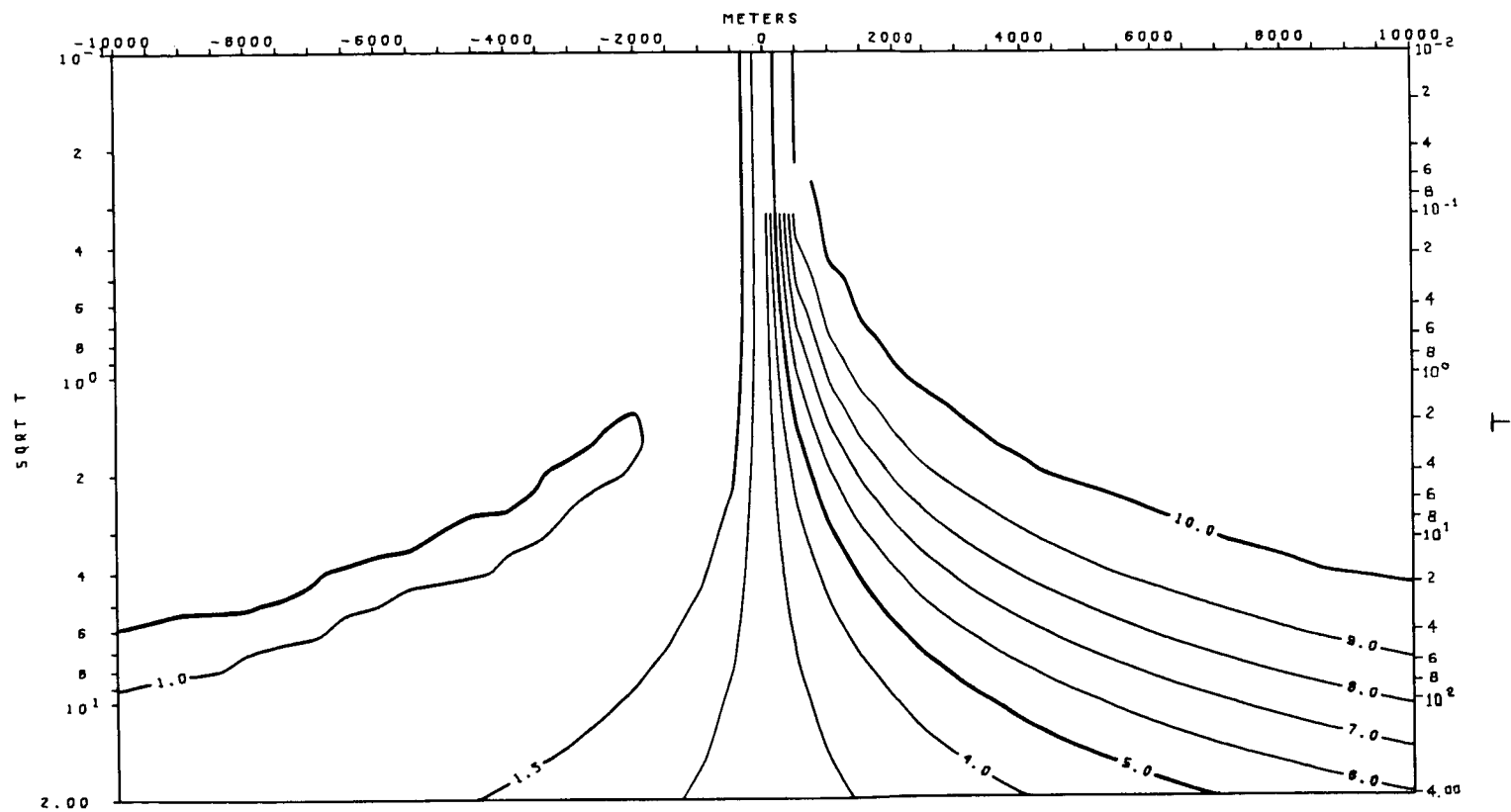
TE MODE APPARENT RESISTIVITY VS. PERIOD (T) MODEL 1-b
