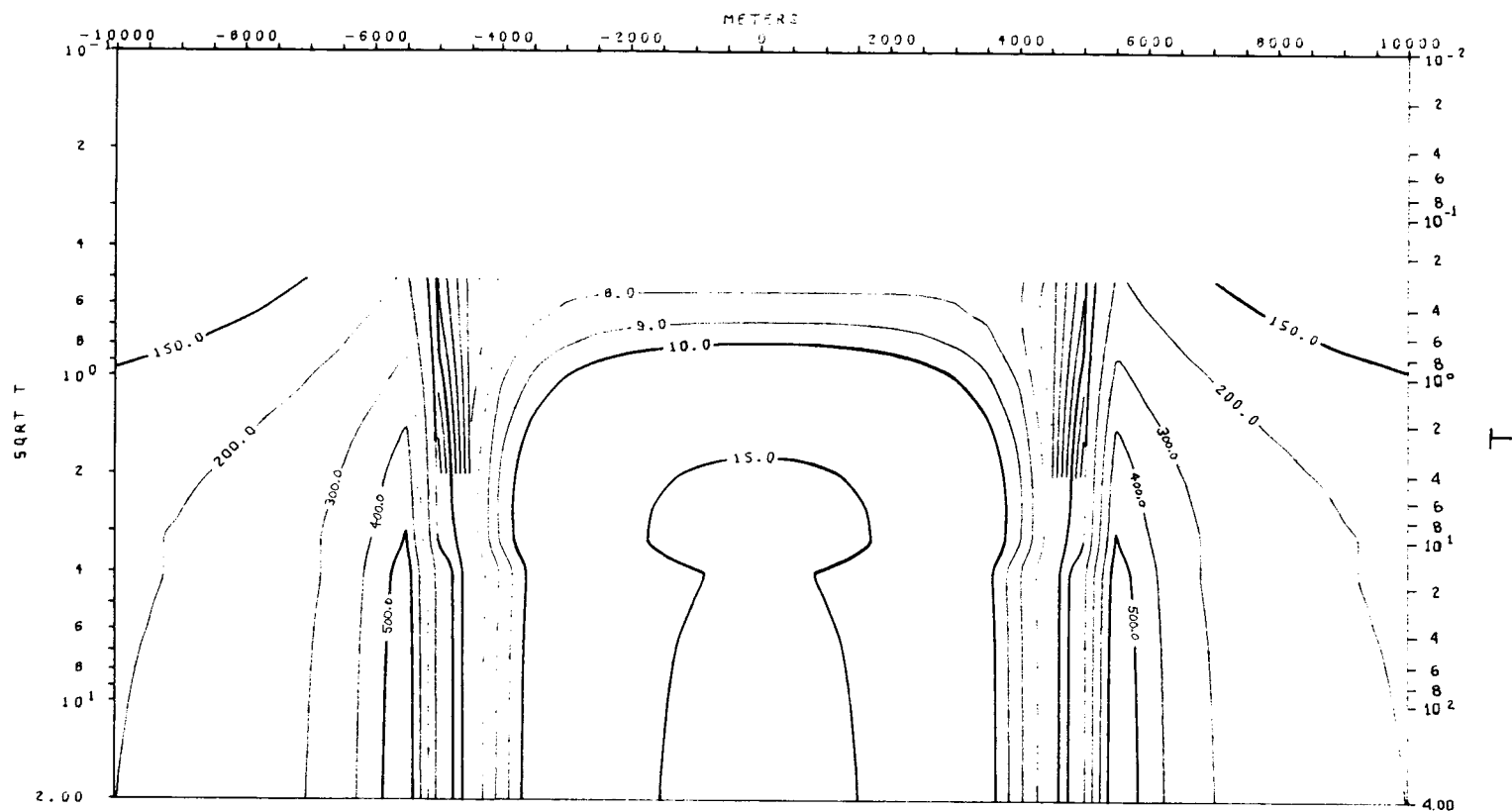
TM MODE APPARENT RESISTIVITY VS. PERIOD (T) MODEL 4-b
