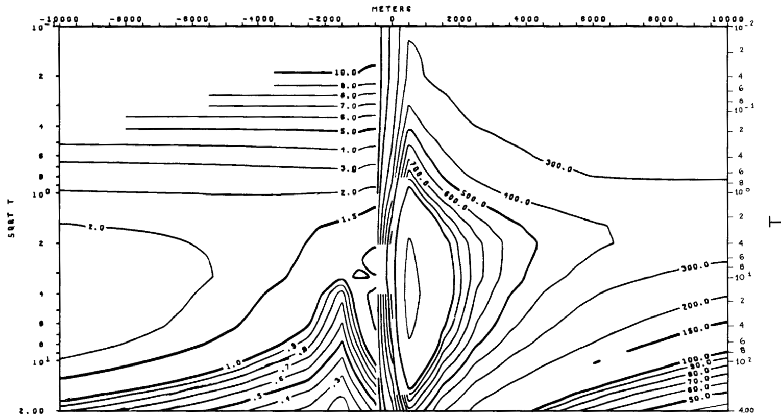
TM MODE APPARENT RESISTIVITY VS. PERIOD (T) MODEL 6-b
