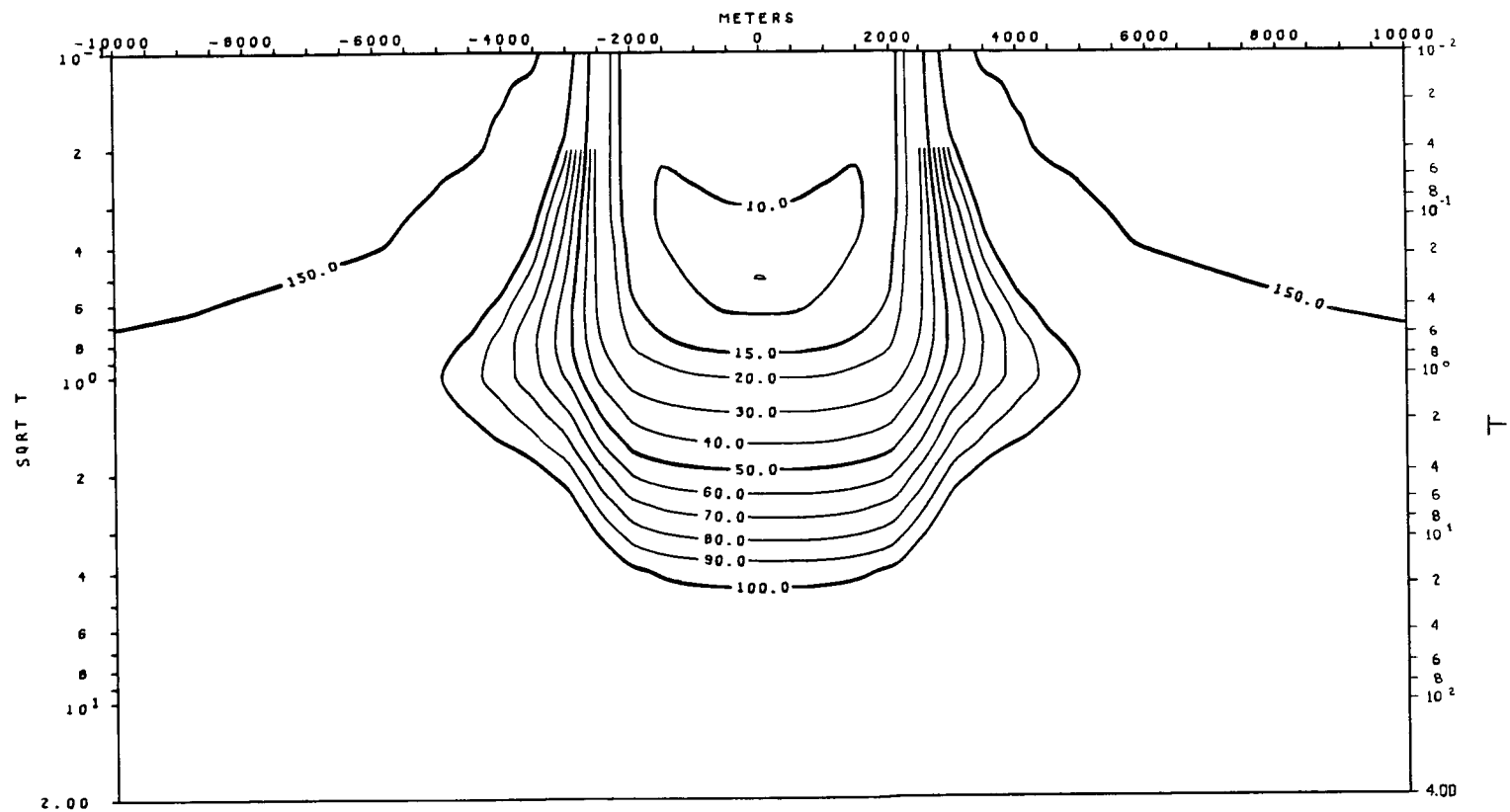
TE MODE APPARENT RESISTIVITY VS. PERIOD (T) MODEL 4-a
