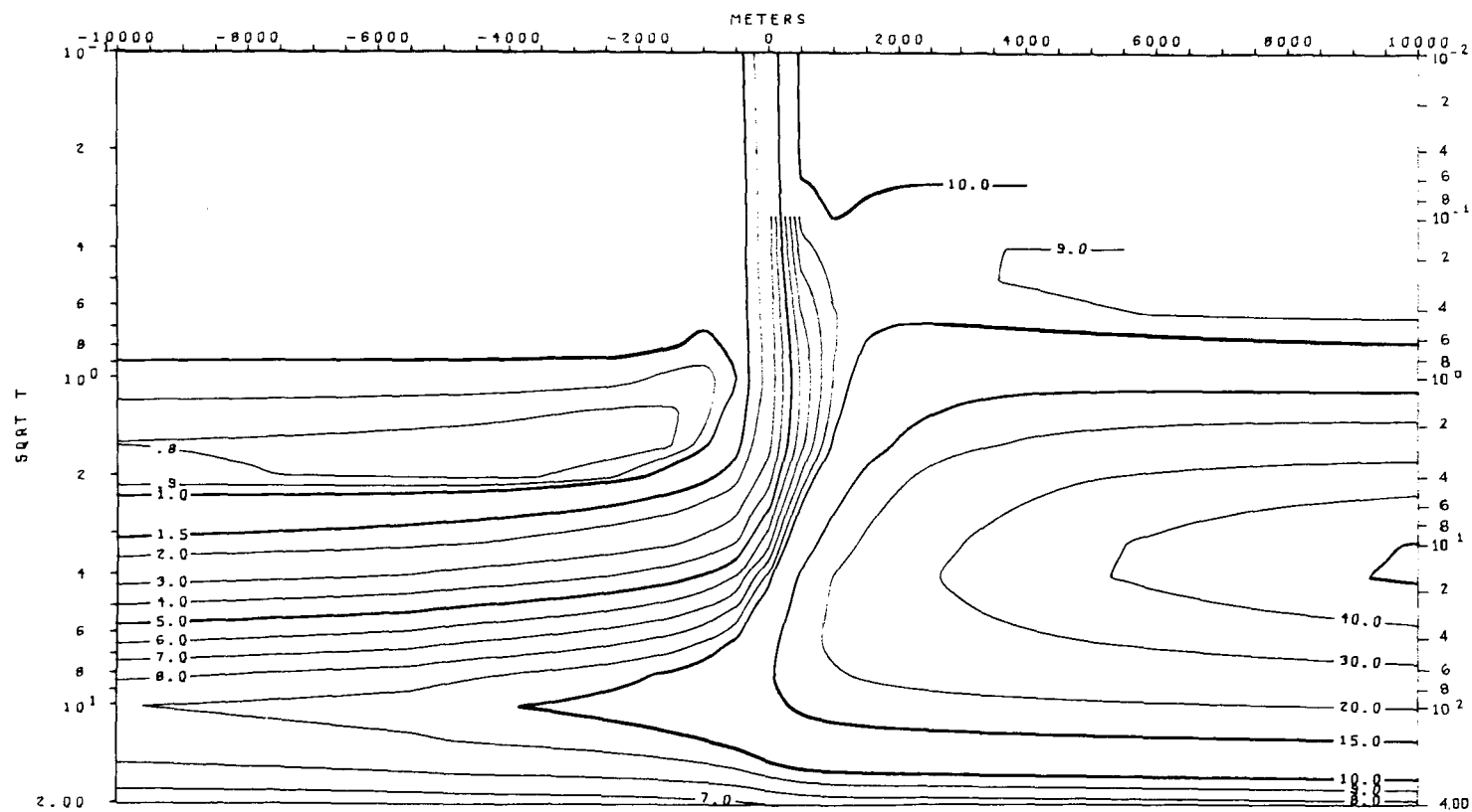
TE MODE APPARENT RESISTIVITY VS. PERIOD (T) MODEL 2-b
