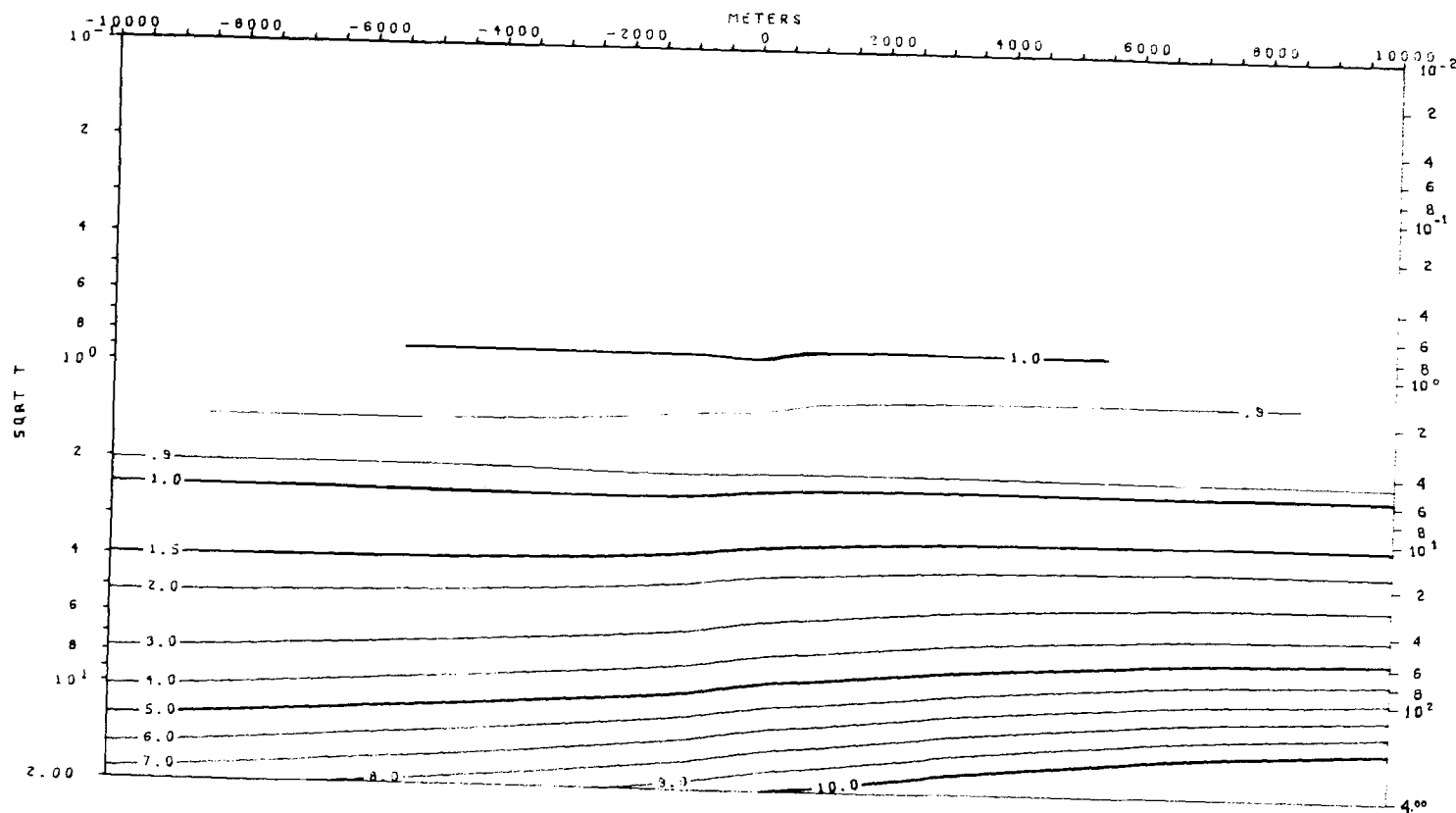
TE MODE APPARENT RESISTIVITY VS. PERIOD (T) MODEL 3-a
