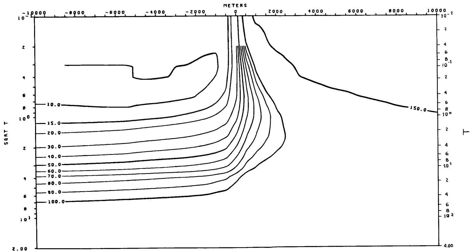
TE MODE APPARENT RESISTIVITY VS. PERIOD (T) MODEL 4-d
