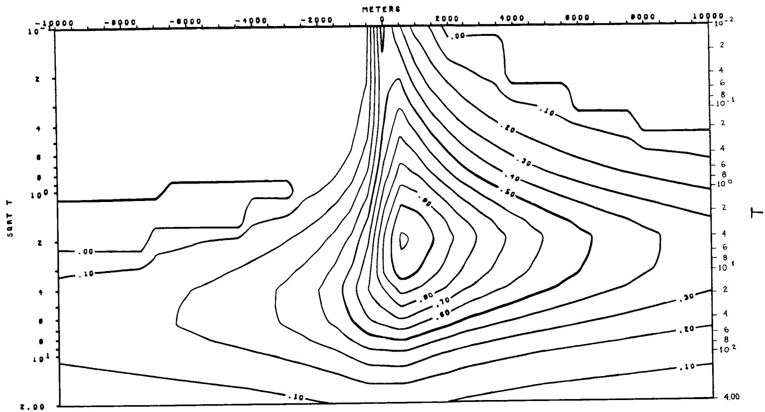
TIPPER VS. PERIOD (T) MODEL 6-b
