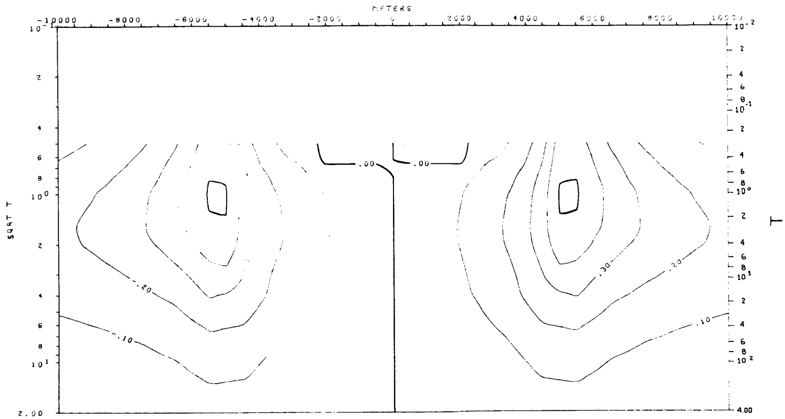
TIPPER VS. PERIOD (T) MODEL 4-b
