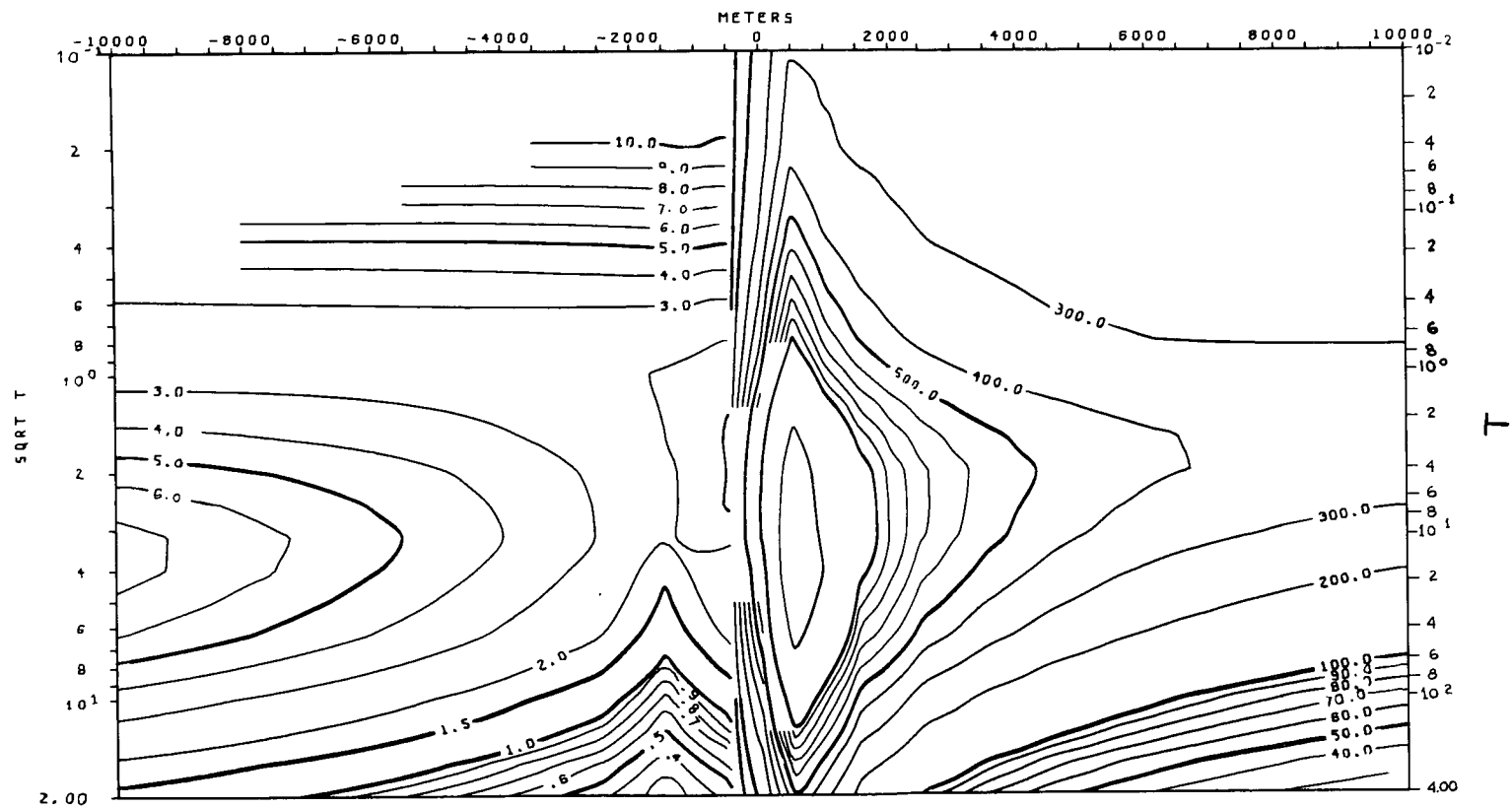
TE MODE APPARENT RESISTIVITY VS. PERIOD (T) MODEL 6-a
