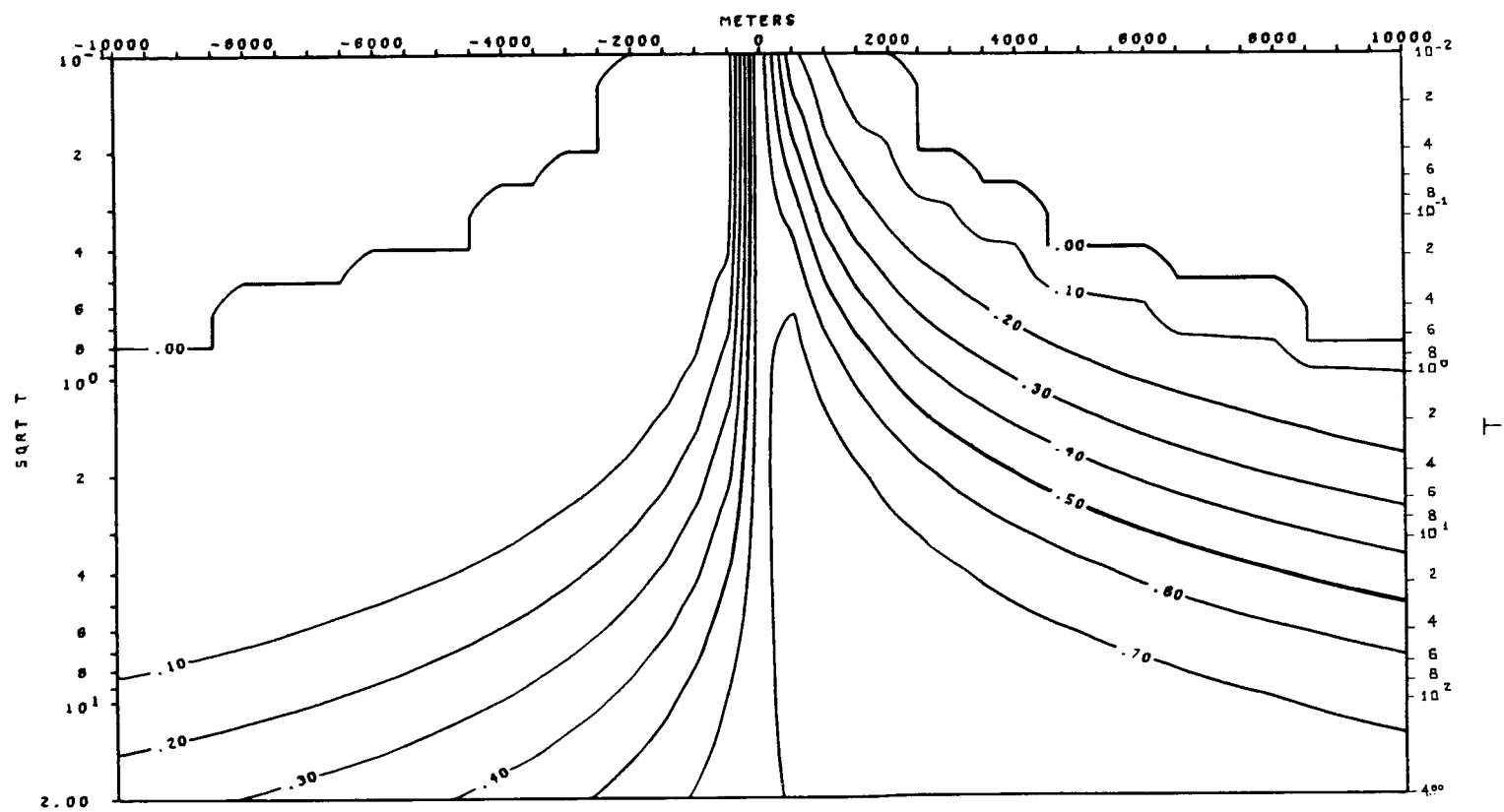
TIPPER VS. PERIOD (T) MODEL 1-a
