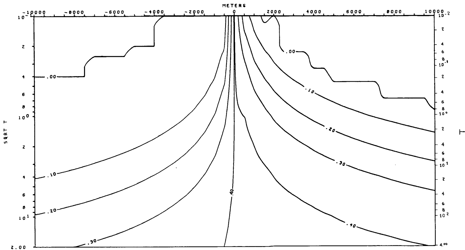
TIPPER VS. PERIOD (T) MODEL 1-c
