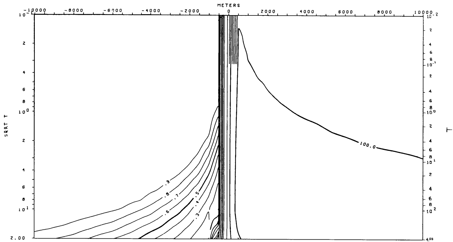
TM MODE APPARENT RESISTIVITY VS. PERIOD (T) MODEL 1-a
