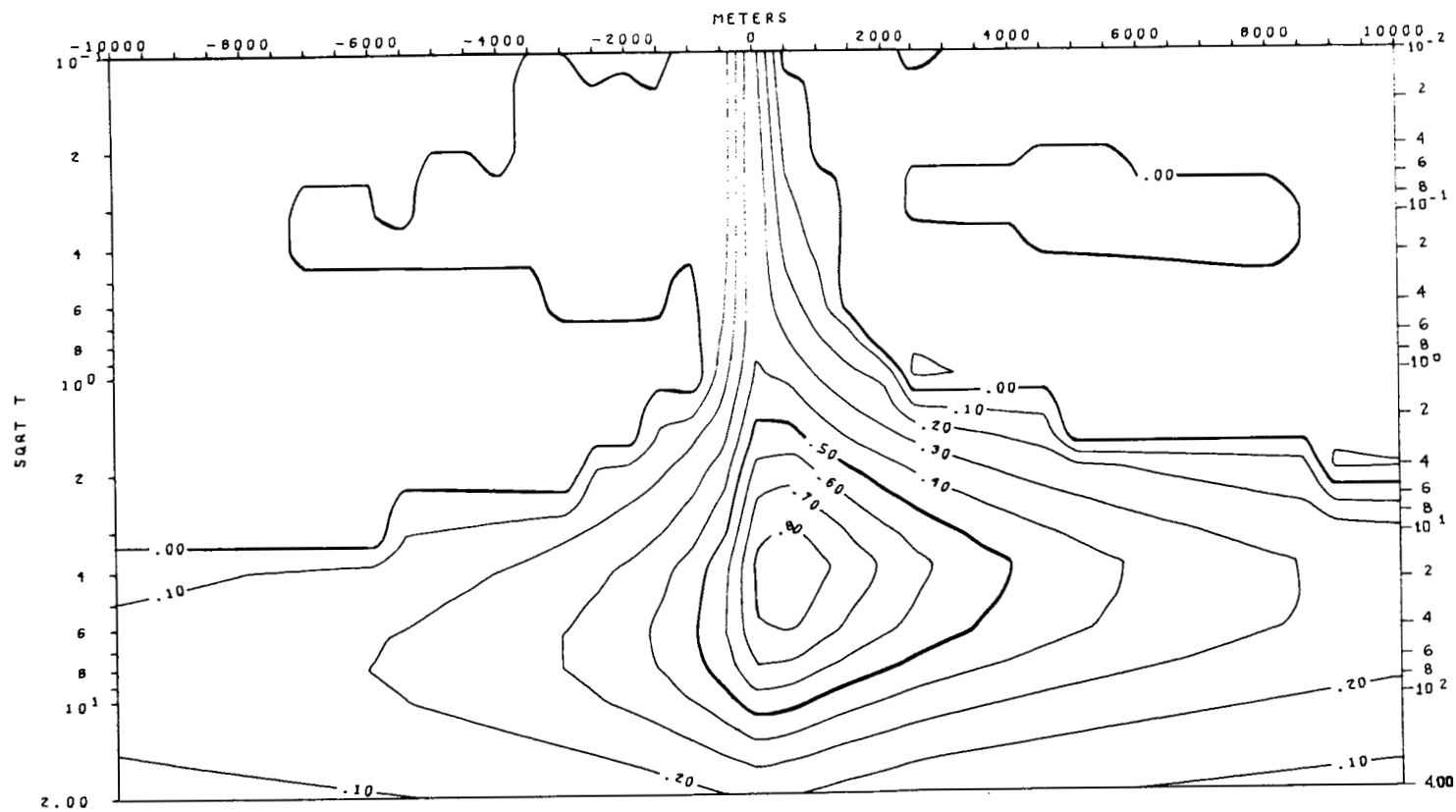
TIPPER VS. PERIOD (T) MODEL 2-b
