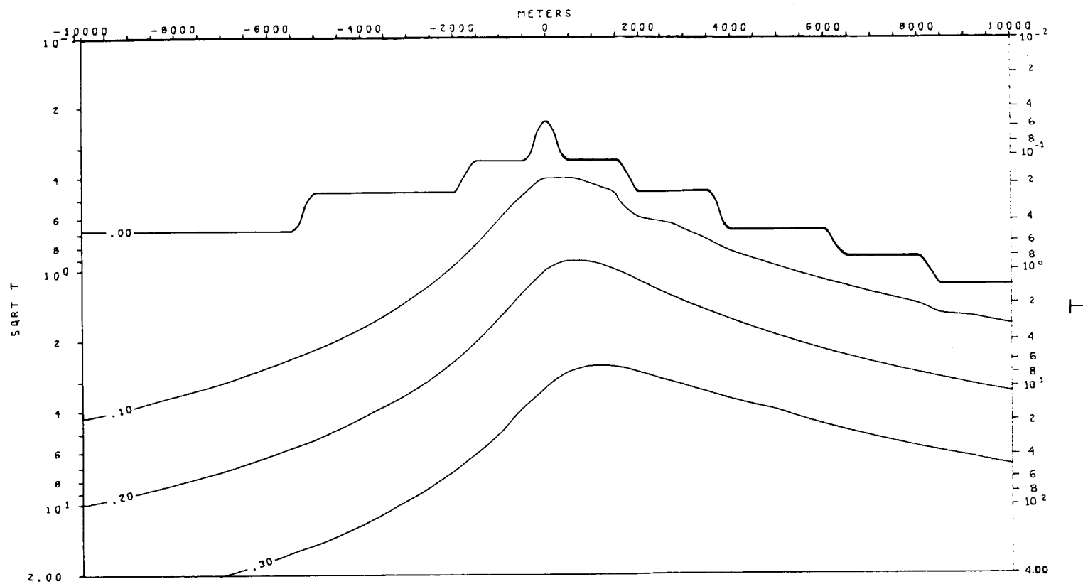
TIPPER VS. PERIOD (T) MODEL 3-c
