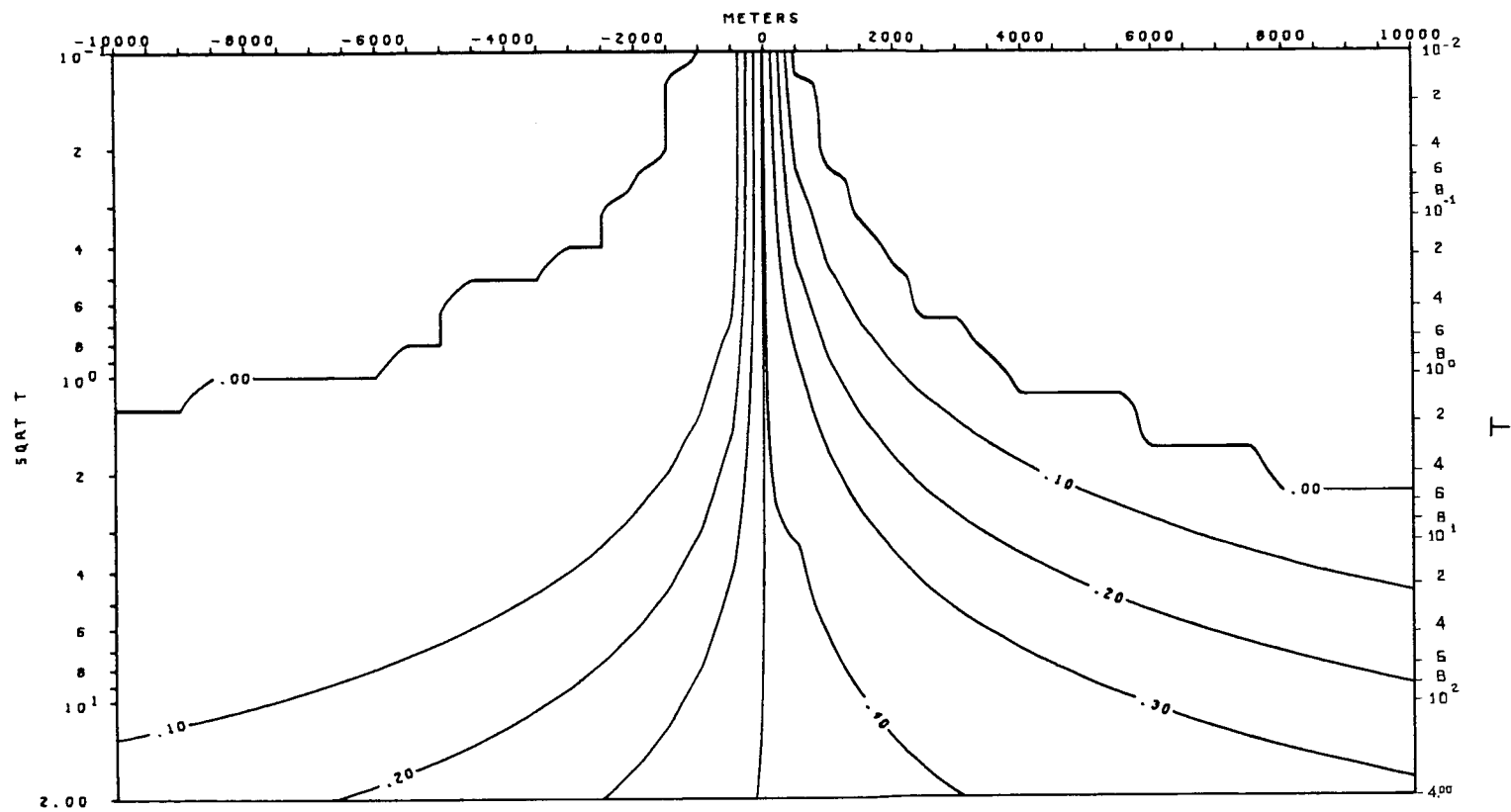
TIPPER VS. PERIOD (T) MODEL 1-b
