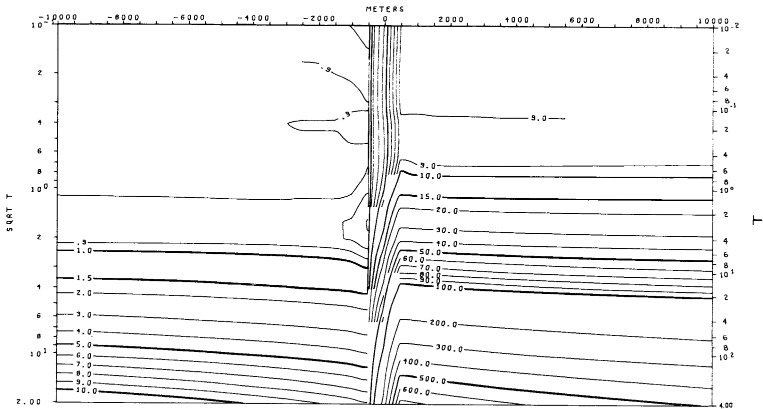
TM MODE APPARENT RESISTIVITY VS. PERIOD (T) MODEL 2-a
