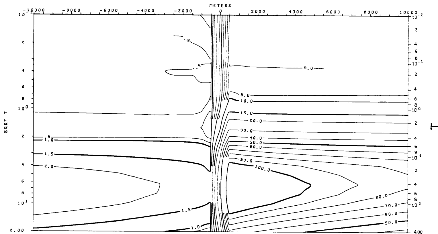
TM MODE APPARENT RESISTIVITY VS. PERIOD (T) MODEL 2-b
