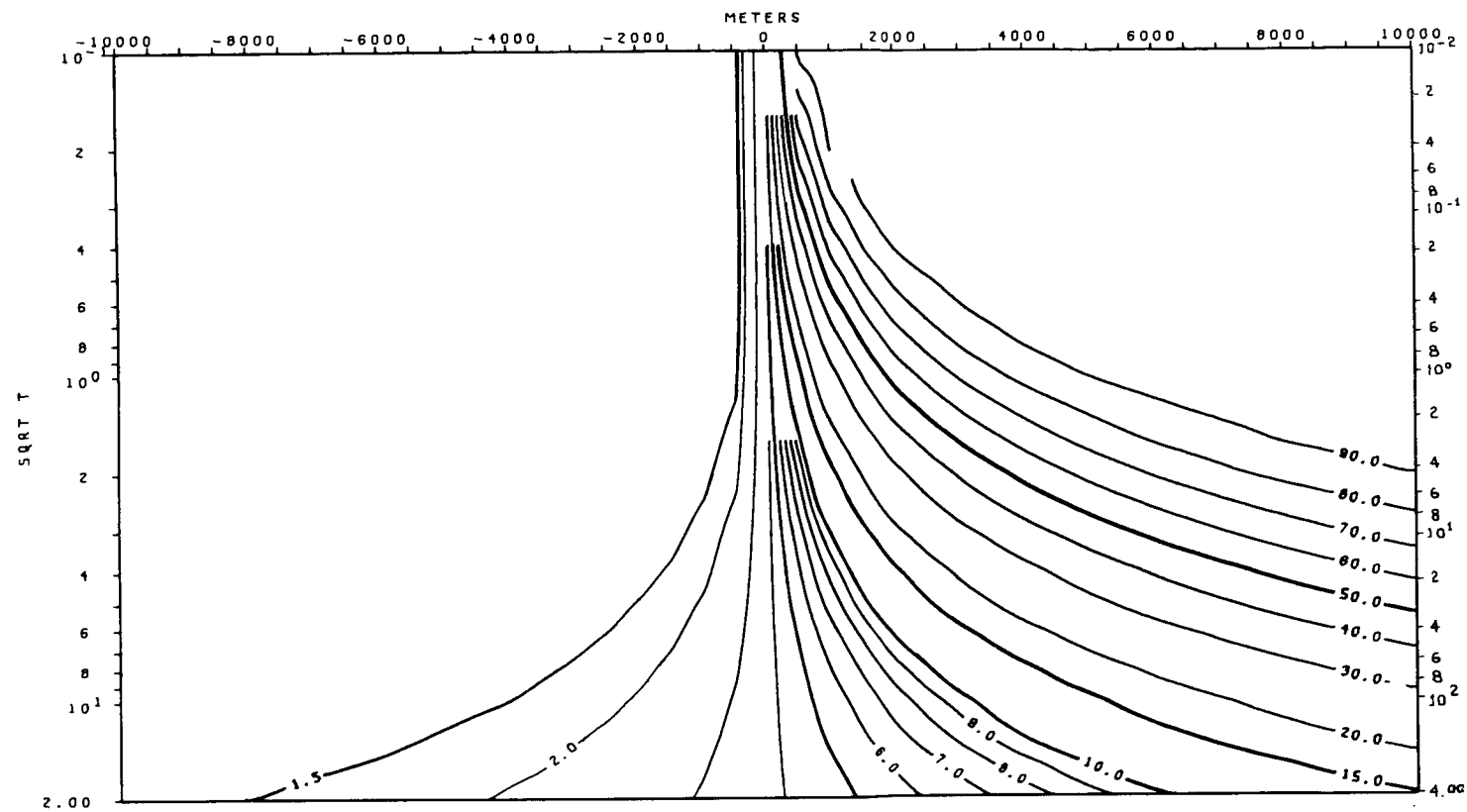
TE MODE APPARENT RESISTIVITY VS. PERIOD (T) MODEL 1-a
