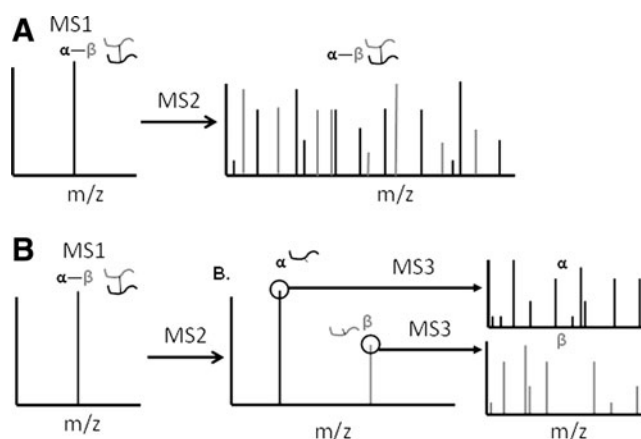
FIG. 4. MS sequencing of inter-linked peptides. (A) MS_2 analysis of a noncleavable inter-linked peptide ( \alpha - \beta ) results in a complex spectrum containing sequence ions from both peptides, which prevents it from being searched effectively by conventional database search engines; (B) MS_2 analysis of an MS-cleavable inter-linked peptide detected in MS_1 , for example, a DSSO cross-linked peptide, results in the physical separation of \alpha and \beta peptides, which enables their subsequent MS_3 sequencing for unambiguous identification using conventional database search engines. DSSO, disuccinimidyl sulfoxide; MS, mass spectrometry.
