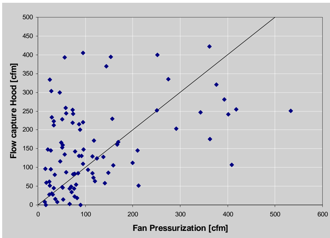
Figure A1. Comparison of total duct leakage predictions using flow capture hood and fan pressurization techniques in single family houses
