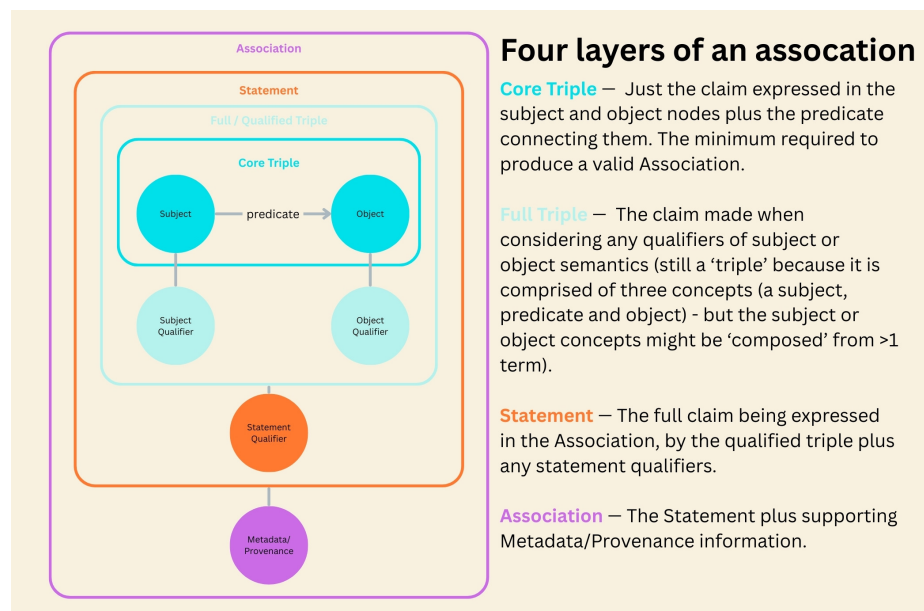
Fig. 1. Biolink Model is based on a nested structure with a core triple in the centre. The subject and object in the triple can be qualified. The whole statement can also receive qualifiers. Everything is wrapped in metadata that provides provenance for the statement. Diagram recreated from Unni et al. 2022 with permission.
