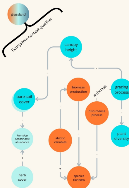
Fig. 4. This diagram shows how the process of encoding papers using the Ecolink Model would function when feeding those papers into a knowledge graph (KG). First, studies are gathered using systematic searching protocols (a). Second, the data is manually or automatically extracted and fitted to the ELM schema in a "semantic parsing" process in which natural language text is translated into an RDF-based syntax using ontology terms, following the structure and constraints in the ELM schema (b). Third, links are established between common node classes (c). Note that (c) is simplified to represent links as + or - for graphical ease. The formal representation would specify whether each node increases or decreases as part of the association.
