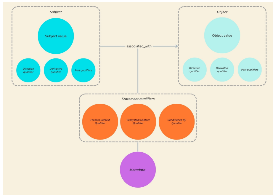
Fig. 2. The overall structure of ELM's association schema. Each circle represents a "slot" in LinkML. This representation shows all possible slots in the schema. Note that the statement qualifiers and metadata apply to the entire association and not simply the edge. It is represented here as attached to the edge because a Neo4j database would model it as such.
