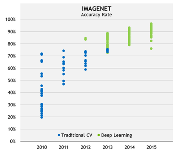
Figure 1: Deep Learning far outperforms traditional computer vision in image recognition. The figure shows the relative performance improvement in error rates on ImageNet's Large Scale Visual Recognition Challenge (ILSVRC) to classify one million images into one thousand categories
