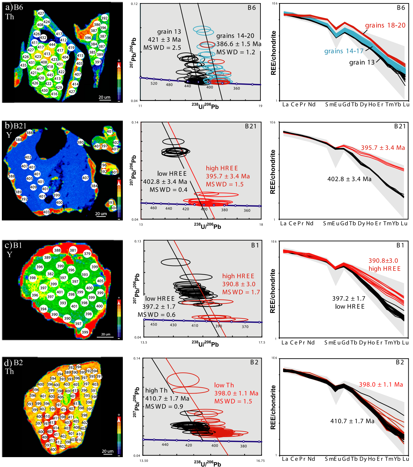
Fig. 6. Examples of monazite with multiple Caledonian dates. a) Different grains in B6 have similar Th zoning, but distinct ages and REE patterns. b) B21 grain core is homogenous in Y, has old ages, low HREE and high common Pb; patchy-zoned rims and smaller grains are younger, have elevated HREE and low common Pb. c) B1 grain core has old ages, low HREE and high common Pb; rims are younger, have elevated HREE and low common Pb. d) B2 grain core has old ages and higher Th; rims are younger and lower in Th [from Holder et al., 2015]. Left: Monazite composition maps determined by X-ray counts; red shows high counts, blue low. Laser spots show “207-corrected” ^{206}\text{Pb}/^{238}\text{U} dates. Middle: Isochrons anchored to Stacey–Kramers common ^{207}\text{Pb}/^{206}\text{Pb} . Right: REE abundances color coded to middle column. Gray field shows entire range of monazite measured in this study. (For interpretation of the references to color in this figure legend, the reader is referred to the web version of this article.)
